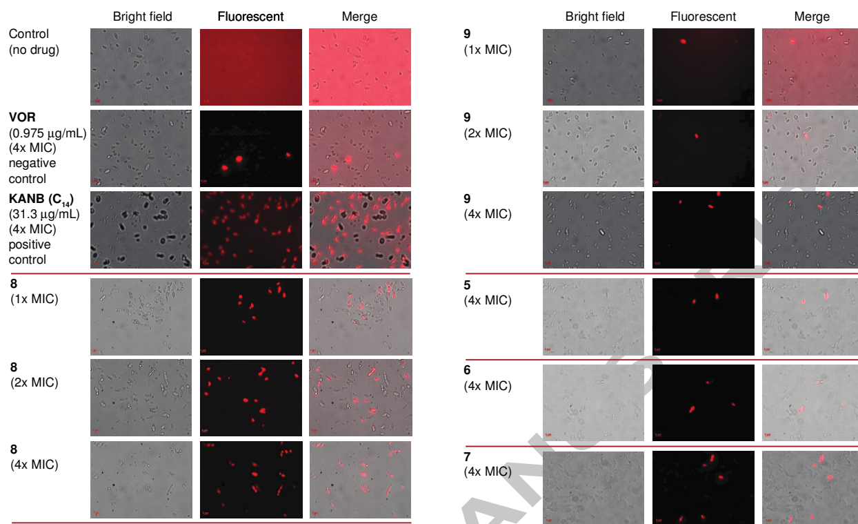
Fig. 6. Effect of the controls VOR (negative) and KANB (C 14 ) (positive) as well as compounds 5-9 on the cell membrane integrity of C. albicans ATCC 10231 (strain A ). For the three columns on the left from top to bottom: Propidium iodide (PI) dye uptake by yeast cells without drug, with VOR (0.975 µg/mL), KANB (C 14 ) (31.3 µg/mL), and compound 8 (1x, 2x, and 4x MIC). For the three columns on the right from top to bottom: Propidium iodide (PI) dye uptake by yeast cells with compound 9 (1x, 2x, and 4x MIC), as well as compound 5 , 6 , and 7 at 4x MIC. The experiments were performed in duplicate.
