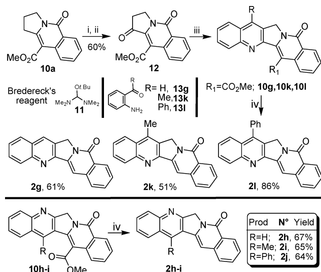
SCHEME 3. Rosettacins 2g–l and Isorosettacins 2h–j a
