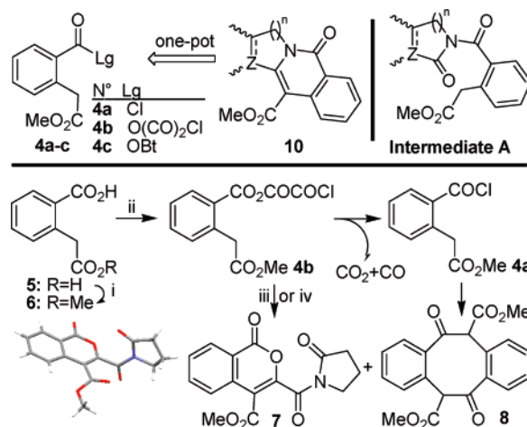
SCHEME 2. Reactivity of 4 and ORTEP Plot of Derivative 7a
