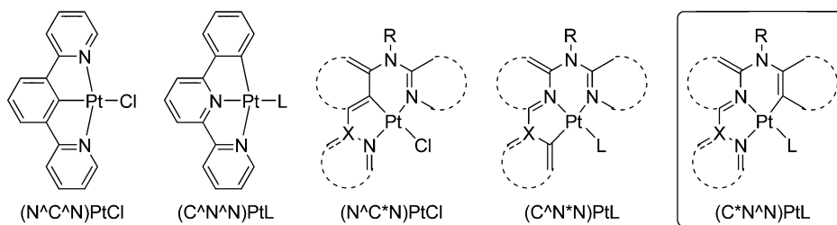
Chart 1. Schematic Representation of N^{\wedge}C^{\wedge}N , C^{\wedge}N^{\wedge}N , N^{\wedge}C^*N , C^{\wedge}N^*N , and C^*N^{\wedge}N -Coordinated Platinum Complexes
