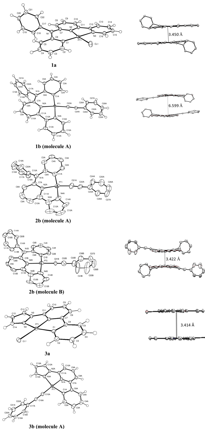
Figure 1. Perspective drawing of 1a and 1b (molecule A), 2b (molecules A and B), and 3a and 3b (molecule A). Ellipsoids are at the 50% probability level. The \pi\cdots\pi contacting distances between two molecules in the crystal packing are shown on the right for 1a , 1b , 2b , and 3a . There was no \pi\cdots\pi interaction in the crystal packing of 3b .
