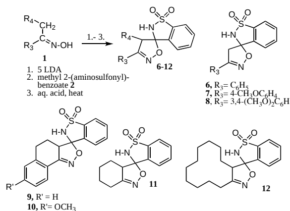
Figure 2. spiro(Benzisothiazole-Isxazole) Dioxides, 6-12 .
