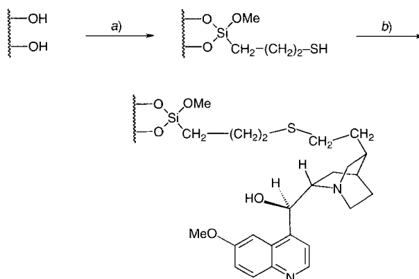
Scheme 3. Chiral Stationary Phase Mode from Silica-Gel-Bound Quinine
