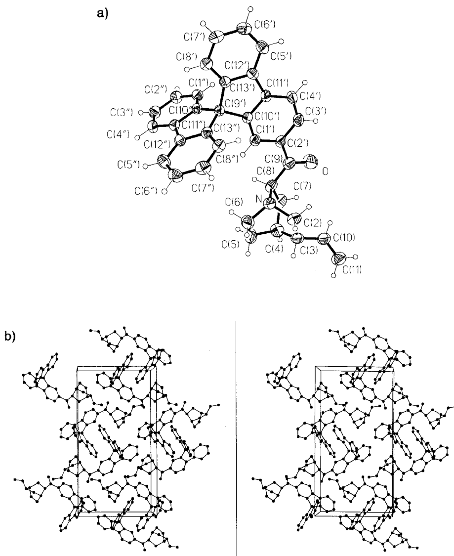
Fig. 3. a) Molecular structure of (+)- 14 . The numbering in use for Cinchona alkaloids is shown. b) Stereoview of the crystal packing of (+)- 14 showing the exclusive edge-to-face aromatic interactions between fluorene rings of neighboring molecules.
