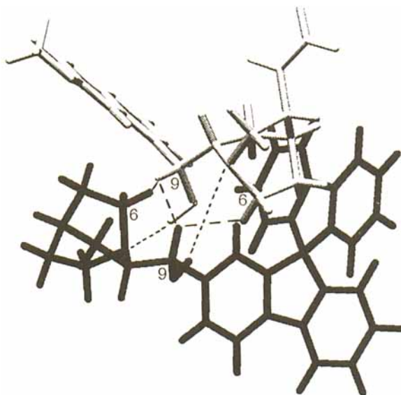
Fig. 10. Computer model of the more stable diastereoisomeric complex formed between (8 R ,9 S )- 5 and quinine ( 1 ). Shown are the three observed intermolecular NOEs (----) and the two host-guest H-bonds (.....).
