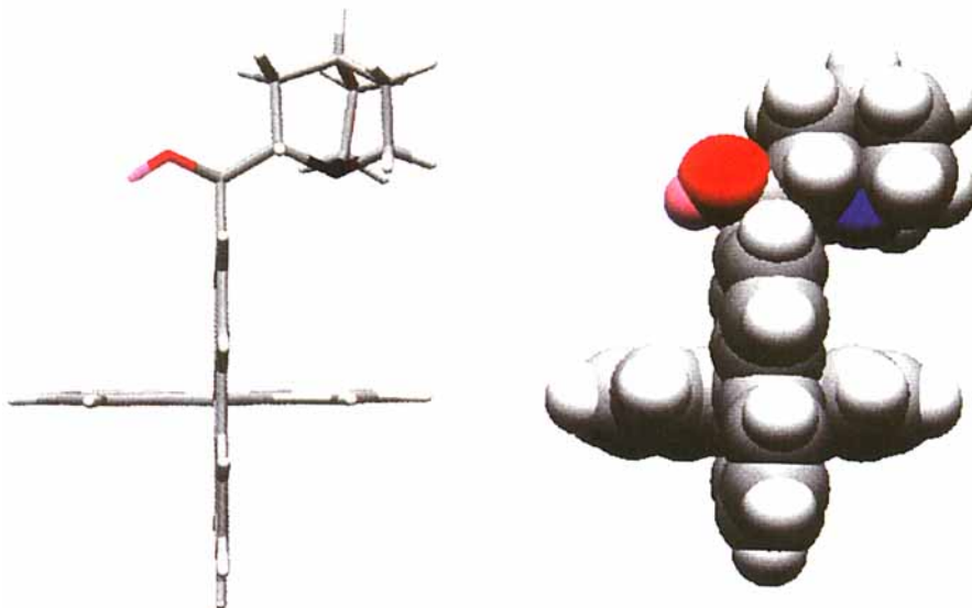
Fig. 6. 'Polytube' (left) and space-filling (right) models of the lowest-energy conformer of (8 S ,9 R )- 5 in \text{CHCl}_3 as revealed in a MC search within MacroModel V. 4.0
