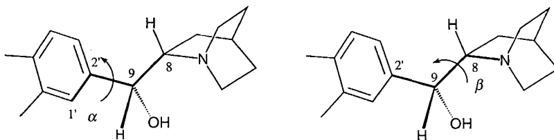
Fig. 5. Definition of the torsional angles \alpha and \beta in (8S,9R) -5
