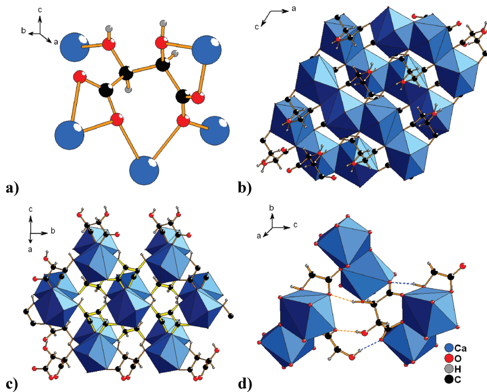
Figure 3. Views of \text{Ca}(\text{m-Tar}) ( 7 ). (a) Metal–tartrate coordination. (b) View down the b axis, showing the 1-D edge-sharing \text{M–O–M} chains. (c) View down the [101] axis, showing the tartrate ligands (yellow bonds) linking each \text{M–O–M} chain to six others. (d) Hydrogen bonding showing two crystallographically unique hydrogen bonds (yellow dashed bonds). Dashed bonds in blue are symmetry equivalent to yellow bonds.
