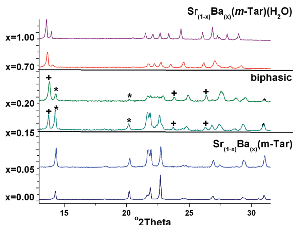
Figure 10. Powder X-ray diffraction patterns of solid solutions of \text{Sr}_{(1-x)}\text{Ba}_x(\text{m-Tar})(\text{H}_2\text{O}) and \text{Sr}_{(1-x)}\text{Ba}_x(\text{m-Tar}) . In the biphasic region, the + symbol indicates characteristic peaks of the \text{Ba}(\text{m-Tar})(\text{H}_2\text{O}) phase; the * symbol indicates characteristic peaks of the \text{Sr}(\text{m-Tar}) phase.
