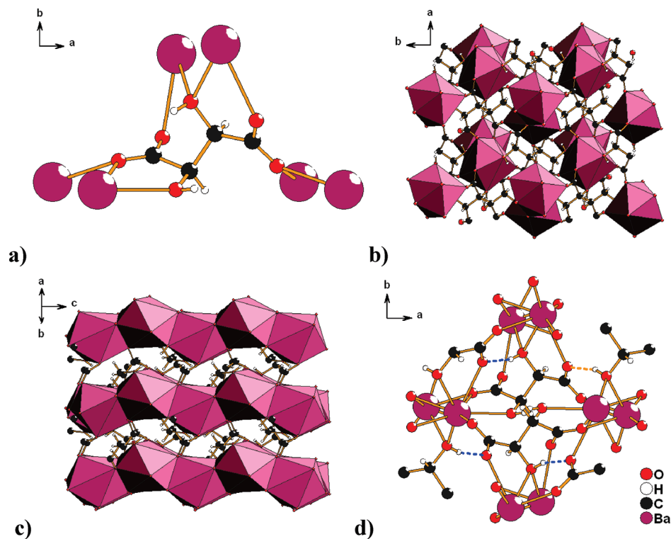
Figure 7. Views of Ba(L-Tar) ( 14 ). (a) Metal–tartrate coordination. (b) View down the c axis showing an end view of the 1-D M–O–M chains. (c) View down the [101] axis showing the M–O–M chains. (d) Hydrogen bonding showing one crystallographically unique bond (dashed yellow bonds). Dashed bonds in blue are symmetry equivalents.
