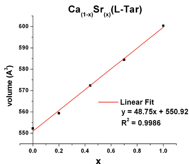
Figure 6. Plot of volume (Å 3 ) versus composition for Ca (1-x) Sr (x) (L-Tar) solid solutions. Cell parameters were determined by Reitveld refinement using GSAS/EXPGUI, 35,36 and composition was determined by ICP.
