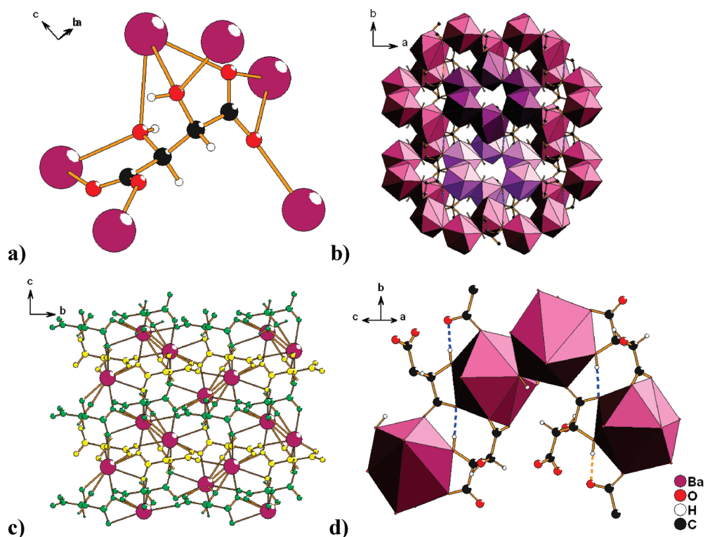
Figure 8. Views of Ba(D,L-Tar) ( 17 ). (a) Metal–tartrate coordination. (b) View of M–O polyhedra with two of the six-membered M–O–M rings tinted as a visual aid. (c) View of the structure down the a axis showing segregation of the L- (yellow) and D-tartrates (green) into separate layers. (d) Hydrogen bonding showing one crystallographically unique hydrogen bond (dashed yellow bond) from a hydroxy group to a carboxylate oxygen. Dashed blue bonds are symmetry-equivalent hydrogen bonds.
