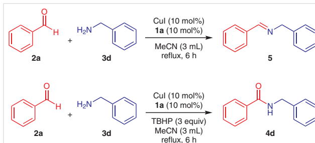
Scheme 3 Control experiments
