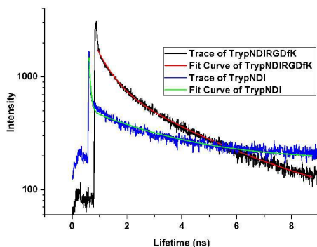
Figure 4. Two-photon time-correlated single photon counting fluorescence decay traces and corresponding fitted curves for the lifetime determinations ( \lambda_{\text{ex}} = 810 nm, TrpNDI 2 , TrpNDIRGDfK 4 , 10 mM, pure DMSO, 5.7 mW).
