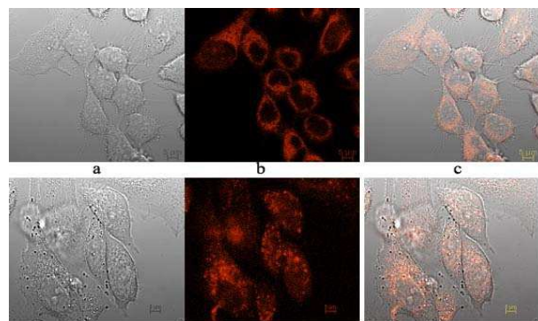
Figure 3. Single-photon laser-scanning confocal microscopy ( \lambda_{\text{ex}} = 543 nm, observed emission: 605–675 nm) of PC-3 cells incubated for 25 mins at 37 °C with: (a–c) Compound 2 (100 \mu\text{M} in 1: 99 % DMSO: serum free medium); (d–f) Compound 4 (100 \mu\text{M} in 1: 99 % DMSO: serum free medium). Scalebar 5 \mu\text{m} . The biolocalisation of 2 is uniform throughout the cytoplasm whereas that of 4 occurs mainly in punctuated, vesicular regions in the cytoplasm.
