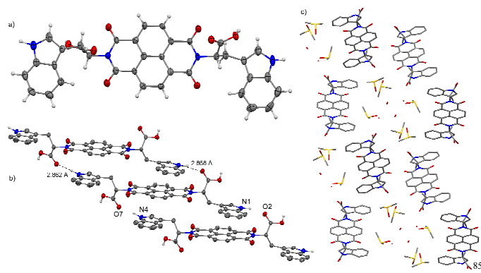
Figure 1. Molecular structure of Compound 2 : (a) Side and (b) crystal unit cell packing views of TrpNDI where all hydrogen atoms and a disordered solvent molecule (DMSO) have been removed for clarity. (c) a view along the a axis rotated by 90° in the b/c plane showing disordered H 2 O and DMSO solvating molecules.
