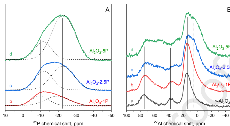
Fig. 6. ^{31}\text{P} MAS NMR (A) and ^1\text{H}\text{-}^{27}\text{Al} CP/MAS NMR (B) spectra of (a) parent \gamma\text{-Al}_2\text{O}_3 , and (b) \text{Al}_2\text{O}_3\text{-1P} , (c) \text{Al}_2\text{O}_3\text{-2.5P} , and (d) \text{Al}_2\text{O}_3\text{-5P} phosphatized alumina supports.
