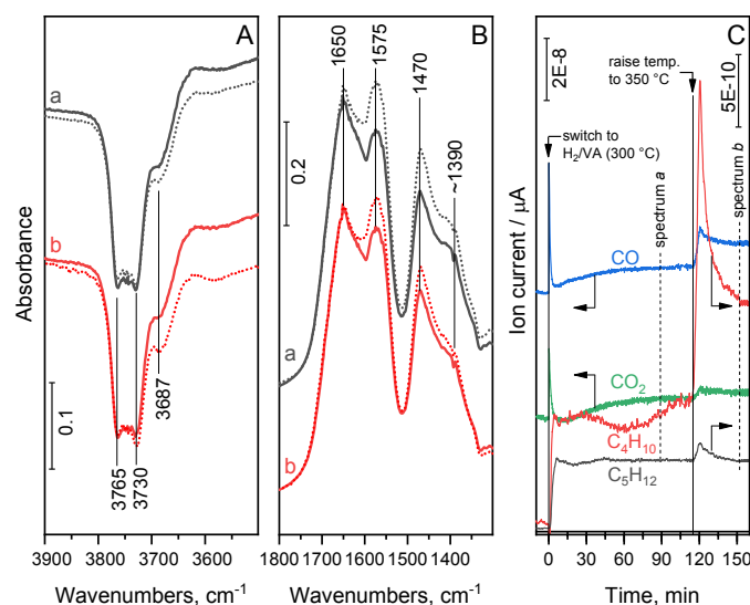
Fig. 9. Difference DRIFT spectra in the range of the (A) O–H stretching and (B) C=O stretching and C–H deformation vibrations on the Pd/Al 2 O 3 catalyst in contact with (a) He/valeric acid mixture (dotted lines) or H 2 /valeric acid mixture (solid lines) at 300 °C or (b) at 350 °C. Part (C) shows the MS signals characteristic of CO, CO 2 , butane, and pentane as HDO products in the effluent gas from the DRIFT reactor cell during the operando DRIFTS experiment with H 2 /valeric acid mixture. Dashed lines indicate the point where spectra were collected after reaching the steady state at the given reaction temperature.
