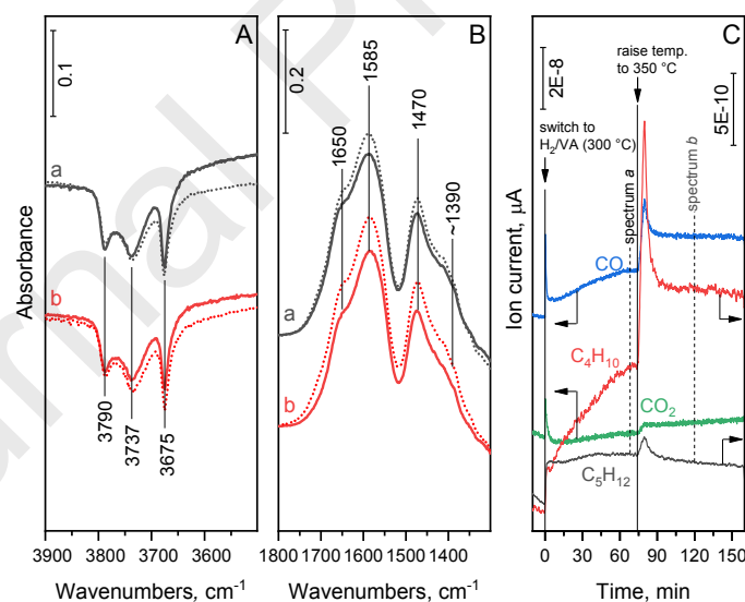
Fig. 10. Difference DRIFT spectra in the range of (A) O–H stretching and (B) C=O stretching and C–H deformation vibrations on Pd/Al 2 O 3 -5P catalyst in contact with He/valeric acid mixture (dotted lines) or H 2 /valeric acid mixture (solid lines) at (a) 300 °C and (b) 350 °C. Part (C) shows the MS signals characteristic of CO, CO 2 , butane, and pentane as HDO products in the effluent gas from the DRIFT reactor cell during the operando experiment with H 2 /valeric acid mixture. Dashed lines indicate the point where spectra were collected after reaching the steady state at the given reaction temperature.
