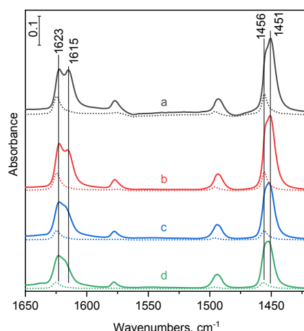
Fig. 5. FT-IR spectra of surface species formed from adsorption of Py on (a) parent \gamma - \text{Al}_2\text{O}_3 , and (b) \text{Al}_2\text{O}_3 -1P, (c) \text{Al}_2\text{O}_3 -2.5P, and (d) \text{Al}_2\text{O}_3 -5P phosphatized alumina supports. Samples were pretreated in situ in the IR cell at 450 °C under high vacuum for 1 h then were contacted with 5 mbar of Py vapor at 200 °C for 30 min. Spectra were taken after evacuation at 100 °C for 30 min (thick solid lines) and then after evacuation at 400 °C for 30 min (thin dotted lines).
