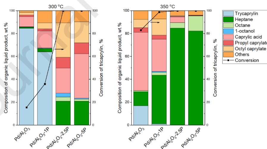
Fig. 8. Catalytic hydroconversion of tricaprylin over Pd catalysts supported on parent \gamma -Al 2 O 3 , and on the Al 2 O 3 -1P, Al 2 O 3 -2.5P, and Al 2 O 3 -5P phosphatized alumina supports. Catalysts were pretreated in situ in H 2 -flow at 450 °C at atmospheric pressure. Catalytic tests were carried out at 300 °C (left) or 350 °C (right) at a total pressure of 21 bars and at a WHSV of 4 g tricaprylin g catalyst -1 h -1 , whereas the H 2 /tricaprylin molar ratio was 20.
