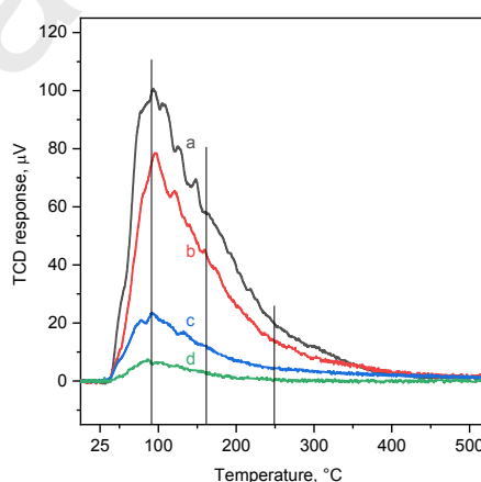
Fig. 4. CO 2 -TPD curves measured for (a) parent \gamma -Al 2 O 3 , and (b) Al 2 O 3 -1P, (c) Al 2 O 3 -2.5P, and (d) Al 2 O 3 -5P phosphatized alumina supports. Prior to the CO 2 -TPD run the sample was activated in O 2 stream at 550 °C. Adsorption was carried out at room temperature at 133 mbar CO 2 pressure. The TPD run was performed in He flow at a heating rate of 10 °C min -1 up to 700 °C.
