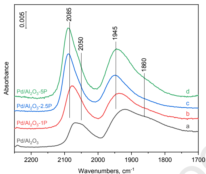
Fig. 7. FT-IR spectra of adsorbed species formed from carbon monoxide on (a) Pd/Al 2 O 3 , (b) Pd/Al 2 O 3 -1P, (c) Pd/Al 2 O 3 -2.5P, and (d) Pd/Al 2 O 3 -5P catalyst samples. Samples were pretreated in situ in the IR cell at 450 °C in H 2 -flow for 1 h then contacted with 5 mbar of CO at room temperature for 30 min. Spectra were taken after removing gas phase CO from the cell by evacuation at room temperature.
