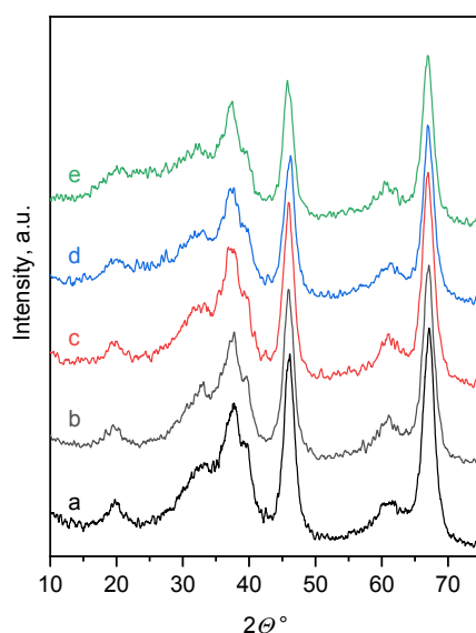
Fig. 1. XRD patterns of (a) parent \gamma - \text{Al}_2\text{O}_3 , and (b) \text{Pd}/\text{Al}_2\text{O}_3 , (c) \text{Pd}/\text{Al}_2\text{O}_3 -1P, (d) \text{Pd}/\text{Al}_2\text{O}_3 -2.5P, and (e) \text{Pd}/\text{Al}_2\text{O}_3 -5P catalyst samples.
