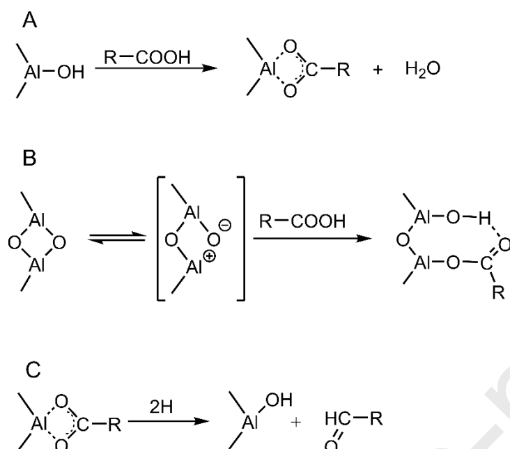
Scheme 2. Formation of carboxylate species via the reaction of carboxylic acid with (A) surface OH groups, (B) Lewis acid ( \text{Al}^{\oplus} ) – Lewis base (O) pair sites, and (C) possible formation of aldehyde intermediate from bidentate carboxylate species.
