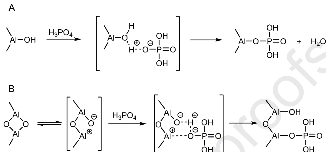
Scheme 1. Reaction of phosphoric acid with (A) surface OH groups, and (B) Lewis acid ( \text{Al}^\oplus ) – Lewis base (O) pair sites.
