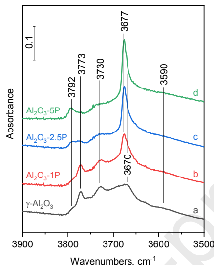
Fig. 2. FTIR spectra of the \nu_{\text{OH}} stretching region of (a) parent \gamma\text{-Al}_2\text{O}_3 , and (b) \text{Al}_2\text{O}_3\text{-1P} , (c) \text{Al}_2\text{O}_3\text{-2.5P} , and (d) \text{Al}_2\text{O}_3\text{ 5P} phosphatized alumina supports. The samples were pretreated in situ in the IR cell at 450\text{ }^\circ\text{C} under high vacuum for 1 h.
