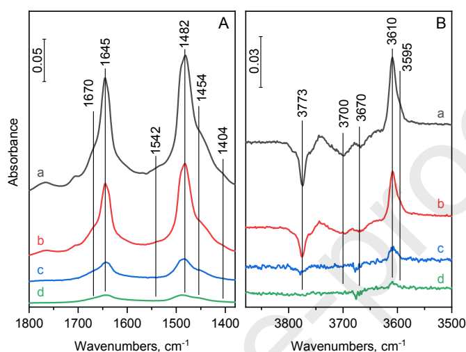
Fig. 3. FTIR spectra of (A) surface species formed from \text{CO}_2 on the parent \gamma\text{-Al}_2\text{O}_3 (a) and on the \text{Al}_2\text{O}_3\text{-1P} (b), \text{Al}_2\text{O}_3\text{-2.5P} (c), and \text{Al}_2\text{O}_3\text{-5P} (d) phosphatized alumina supports and (B) the corresponding difference spectra in the range of the O–H stretching vibrations. Samples were pretreated in situ in the IR cell at 450\text{ }^\circ\text{C} under high vacuum for 1 h then were contacted with 15 mbar of \text{CO}_2 at room temperature for 30 min. Spectra were taken after 30 min evacuation at room temperature.
