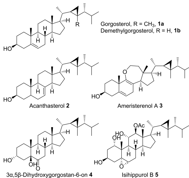
Figure 1. Structures of Gorgosterol ( 1a ), Demethylgorgosterol ( 1b ), and selected derivatives 2–5 .
