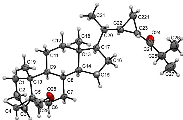
Figure 3. ORTEP-style representation of one of the crystallographic independent molecules of the ketone 8 . Thermal ellipsoids are shown at a 50% probability level. The absolute configuration was determined crystallographically.
