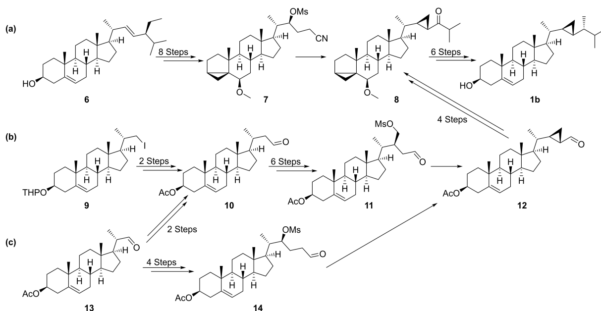
Scheme 1. Previous semisyntheses of demethylgorgosterol ( 1b ). Routes developed by (a) Djerassi et al. [17] and (b), (c) Ikekawa et al. [18]
