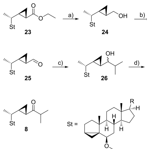
Scheme 5. Transformation of ester 23 into the known ketone 8 in four steps. Reaction conditions: a) LiAlH 4 , THF, reflux, 4 h, quant. b) IBX, DMSO, rt, 16 h, 92 % c) i PrMgBr, THF, –18 °C, 2 h, 83 %. d) PCC, DCM, 2 h, 84 %.
