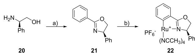
Scheme 3. Synthesis of (R)-Ru-pheox 22 from (R)-2-phenylglycinol ( 20 ). Reaction conditions: a) i) benzoyl chloride, Et 3 N, DCM, 0 °C to rt, 16 h. ii) SOCl 2 , CHCl 3 , 0 °C to rt, 24 h. iii) 2.5 M NaOH, 1,4-dioxan, 0 °C to rt, 4 h, 73 %. b) benzeruthenium(II) chloride dimer, 1 M NaOH, KPF 6 , MeCN, 80 °C, 48 h, 88 %.
