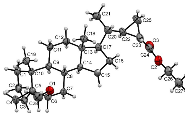
Scheme 2. Synthesis of the alkene 19 starting from commercially available stigmasterol ( 6 ). Reaction conditions: a) TsCl, pyridine, rt, 16 h, quant. b) MeOH, pyridine, reflux, 4 h, 78 %. c) i) O 3 , DCM, MeOH, –78 °C, 45 min; ii) Zn, HOAc, rt, 1 h, 80 %. d) TsNHNH 2 , MS 3 Å, ethanol, rt, 30 min, 50 °C, 30 min, 95 %. e) Dimethyl sulfone, n BuLi, THF, 0 °C to rt, 16 h, 88 %.
