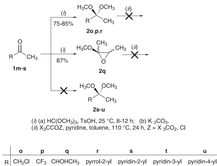
Scheme 2. Limitations of the acetal acylation method.
