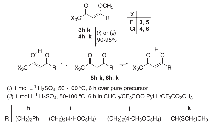
Scheme 5. Hydrolysis of 1,1,1-trifluoro-4-methoxyalk-3-en-2-ones.
