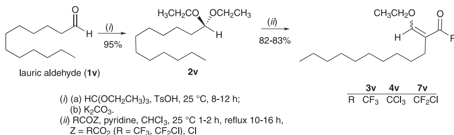
Scheme 4. Acetal acylation applied to 1,1-diethoxydodecane.
