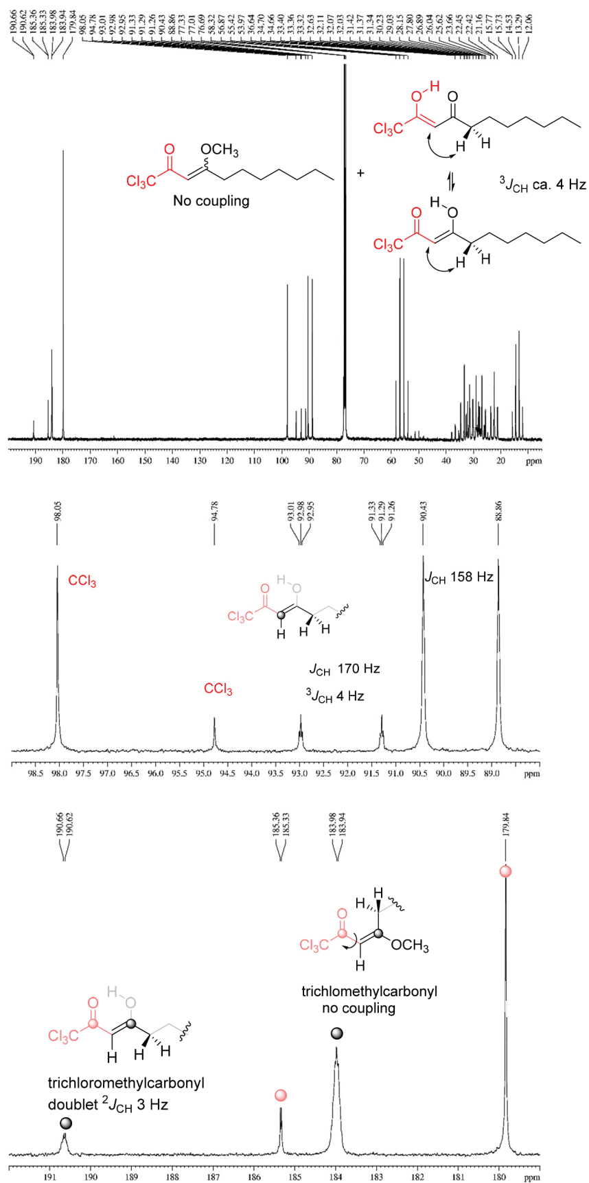
Figure 3. ^{13}\text{C}\{\text{H}\} NMR spectra from mixture 4a + 6a .
