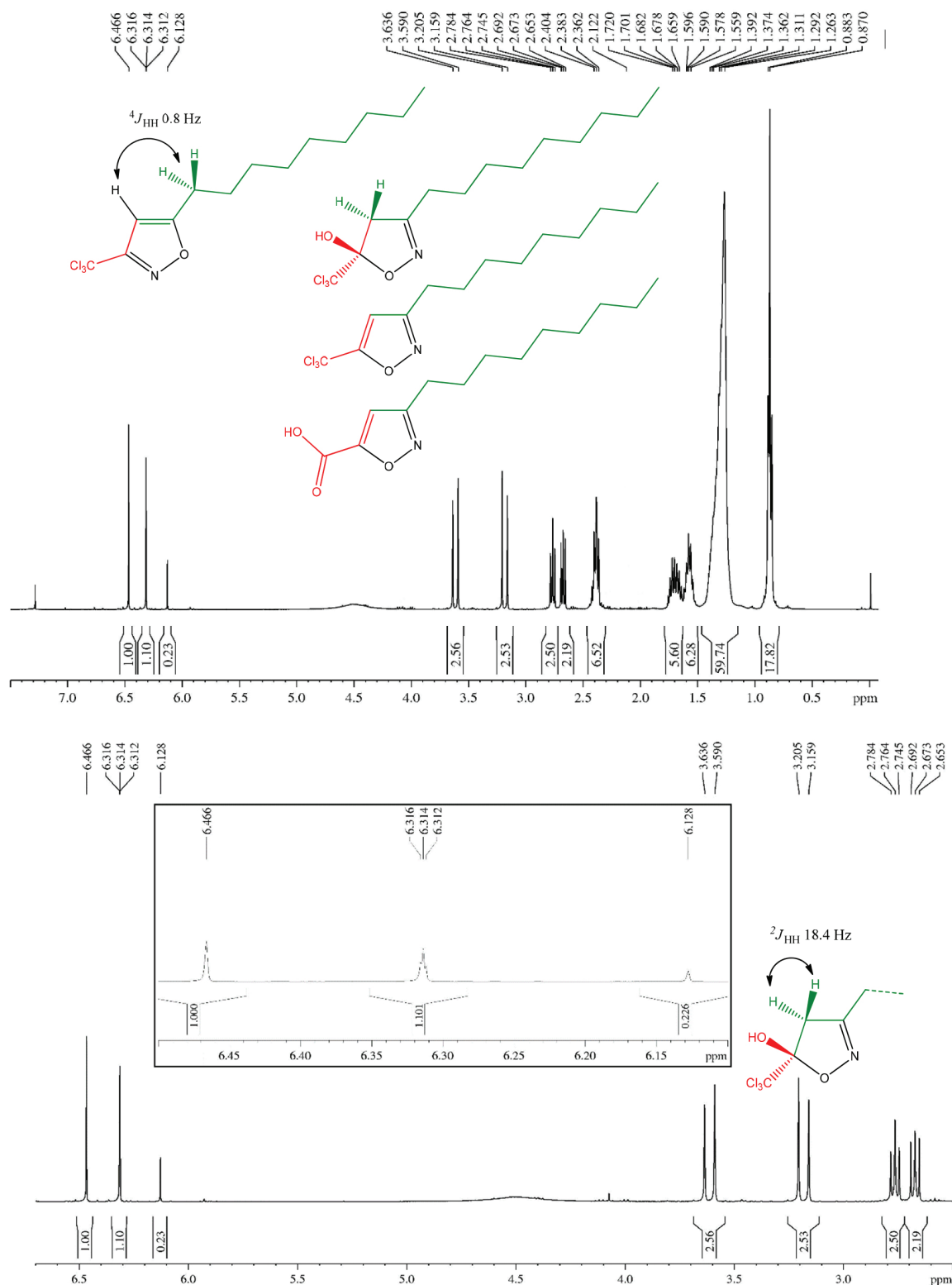
Figure 6. 1 H NMR spectrum of a mixture obtained from a reaction between 4c and NH 2 OH.HCl in 30% H 2 SO 4 .
