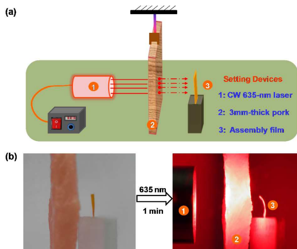
Figure 8. (a) Schematic illustration of the set-up layout of investigating the photoinduced bending behavior of assembly film upon irradiation with CW 635-nm laser (power density = 500 \text{ mW cm}^{-2} ) when a pork with thickness of 3 mm was put between the light source and the assembly film. (b) Photographs of assembly film bending toward the light source in response to the incident light transmitting through the pork (Thickness of each layer in the assembly film: 15 \mu\text{m} of upconverting film and 27 \mu\text{m} of CLCP).
