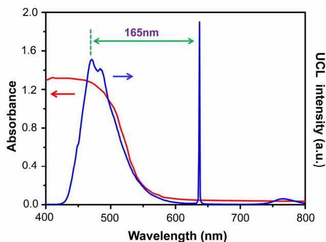
Figure 2. UCL emission spectrum (blue line) of the toluene solution of PtTPBP&BDPPA ( \lambda_{\text{ex}} = 635 nm, power density = 200 \text{ mW cm}^{-2} ) and the UV-Vis absorption spectrum (red line) of the azotolane CLCP film.
