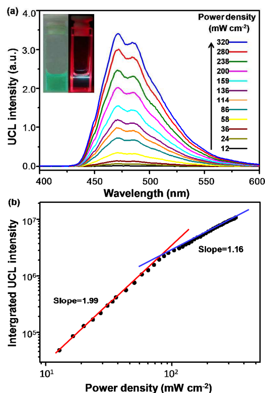
Figure 1. (a) UCL spectra of PtTPBP&BDPPA ([PtTPBP]: 1.0 \times 10^{-5} M and [BDPPA]: 1.5 \times 10^{-3} M) upon excitation of CW 635-nm laser with different incident power densities. Inset: photos of bright-field and photoluminescence emission (without any filter) of PtTPBP&BDPPA inside the 1 cm cuvette ( \lambda_{\text{ex}} = 635 nm). UCL spectra of the toluene solution of PtTPBP&BDPPA at different concentration ratios of PtTPBP to BDPPA were shown in Figure S2 of Supporting Information. (b) Integrated UCL intensity data from part (a) plotted as a function of incident power density. All spectra are measured in de-aerated toluene.
