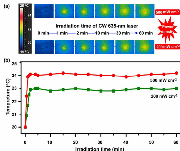
Figure 7. (a) Thermal photographs and (b) temperature changes data from part (a) of the assembly film upon exposure to CW 635-nm laser with two different power densities as a function of irradiation time (Thickness of each layer in the assembly film: 15 \mu\text{m} of upconverting film and 27 \mu\text{m} of CLCP).
