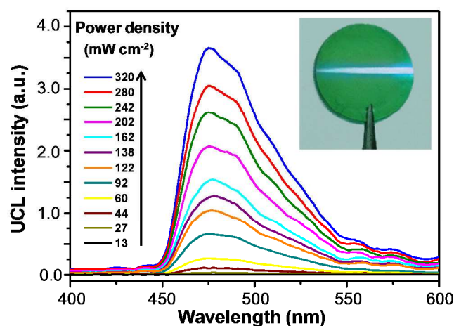
Figure 4. UCL spectra of the upconverting polyurethane film (containing 4 wt% PtTPBP&BDPPA, molar ratio of PtTPBP and BDPPA = 1:150) upon excitation of CW 635-nm laser with different incident power densities. Inset: emission photograph of upconverting polyurethane film with short-pass filter (edge wavelength at 628 nm). UCL spectra of the polyurethane films containing different concentrations of PtTPBP&BDPPA were shown in Figure S9 of Supporting Information.
