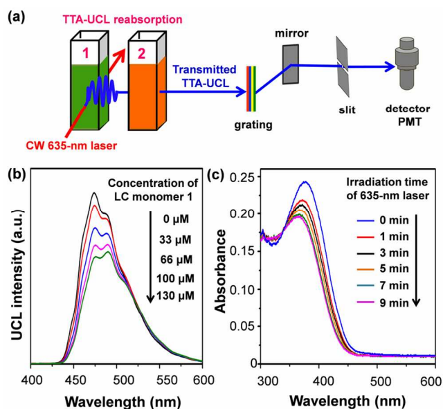
Figure 3. (a) Schematic layout of the UCL emission measurement system. CW 635-nm laser irradiated PtTPBP&BDPPA in cell 1 to trigger TTA-UCL and the generated blue emission went through cell 2 which was filled with the toluene solution of LC monomer 1. The transmitted TTA-UCL emission then passed through the grating instrument system and finally entered the photomultiplier tube (PMT) detector. The excitation laser beam path and the UCL emission pathway are shown in red and blue, respectively. (b) Change in the UCL intensity of transmitted TTA-UCL upon addition of different concentrations of toluene solution of LC monomer 1 in cell 2 under excitation at 635 nm. (power density = 200 \text{ mW cm}^{-2} ) (c) Change in the absorption spectra of the toluene solution of azotolane-containing LC monomer 1 ( 9.0 \times 10^{-6} \text{ M} ) in cell 4 upon irradiation of blue TTA-UCL generated from excitation with CW 635-nm laser in cell 3 (power density = 200 \text{ mW cm}^{-2} ) for different time. (The layout of this UV-Vis absorption measurement system is shown in Figure S6).
