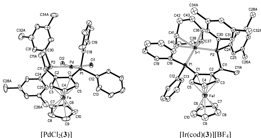
Figure 1. Molecular structures of [\text{PdCl}_2(\text{3})] and [\text{Ir}(\text{cod})(\text{3})][\text{BF}_4] (from ref 21, anion omitted for clarity).
