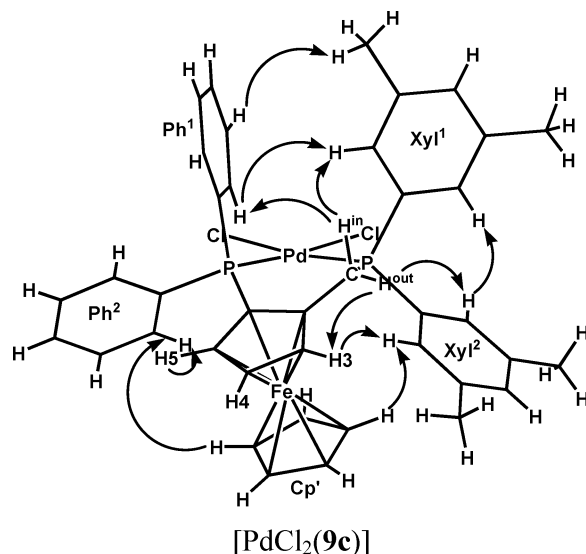
Chart 4. Numbering Scheme and Main NOE Interactions for [PdCl 2 ( 9c )]
