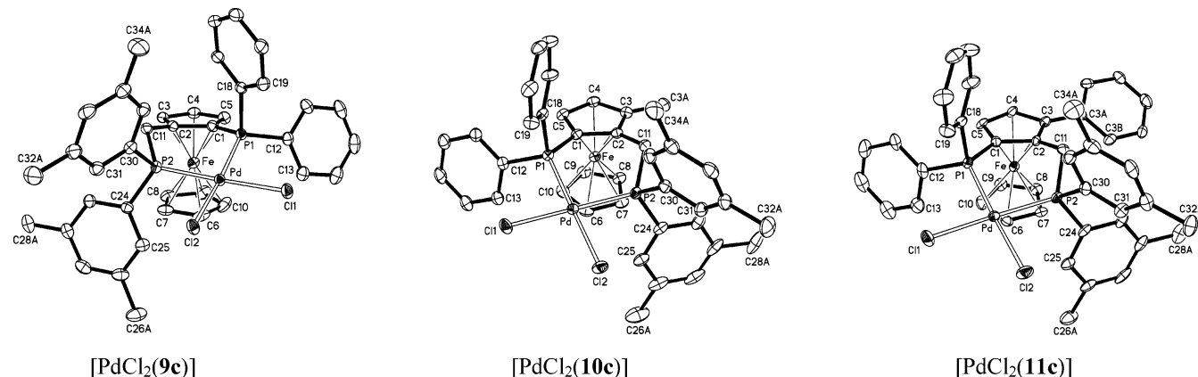
Figure 2. Molecular structures of [\text{PdCl}_2(\text{L})] ( \text{L} = \text{9c} , \text{10c} , and \text{11c} ) in the solid state.
