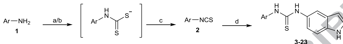
Scheme 1. Synthesis of indolyl thiureas 3-23 . Reagents and conditions: (a) \text{CS}_2 , \text{Et}_3\text{N} , r.t. (b) \text{NaH} , \text{CS}_2 , reflux; (c) \text{Boc}_2\text{O} , DMAP, 0^\circ\text{C} to r.t.; (d) 1H -indole-5-amine, DCM, r.t.
