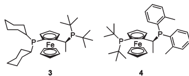
Figure 1. Optimized ligands from screening.
