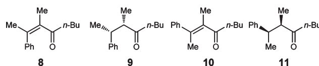
Figure 3. Influence of olefin geometry on stereoinduction.
