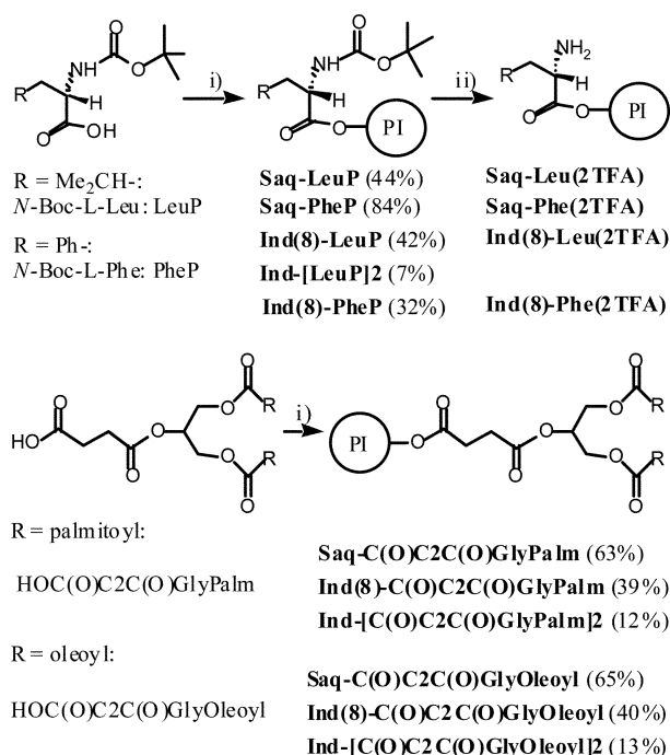
Fig. 2 Synthetic pathway to the ester PI prodrugs derived from L-leucine, L-phenylalanine or from 1,3-diglycerides: i) PI (= Saq or Ind)/EDC/DMAP, \text{CH}_2\text{Cl}_2 or DMF; ii) \text{CF}_3\text{CO}_2\text{H} (TFA)/ \text{CH}_2\text{Cl}_2 , quantitative. Mono- and di-esters of indinavir are obtained during the same reaction. [palmitoyl = \text{CH}_3(\text{CH}_2)_{14} ; oleoyl = ( Z ) \text{CH}_3(\text{CH}_2)_7\text{CH}=\text{CH}(\text{CH}_2)_7 ].
