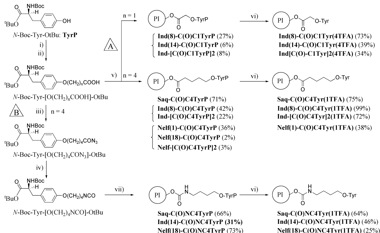
Fig. 3 Synthetic pathway to the (A) ester and (B) carbamate PI prodrugs derived from L-tyrosine: i) \text{Br}(\text{CH}_2)_n\text{CO}_2\text{Et} ( n = 1 or 4 ), \text{K}_2\text{CO}_3 , DMF; ii) LiOH, THF; iii) \text{EtOC(O)Cl} , \text{NaN}_3 , acetone; iv) toluene, \Delta ; v) PI (= Saq, Ind or Nelf)/EDC/DMAP, \text{CH}_2\text{Cl}_2 or DMF; vi) \text{CF}_3\text{CO}_2\text{H} (TFA)/ \text{CH}_2\text{Cl}_2 ; vii) PI (= Saq, Ind, or Nelf), CuCl, \text{CH}_2\text{Cl}_2 or DMF.
