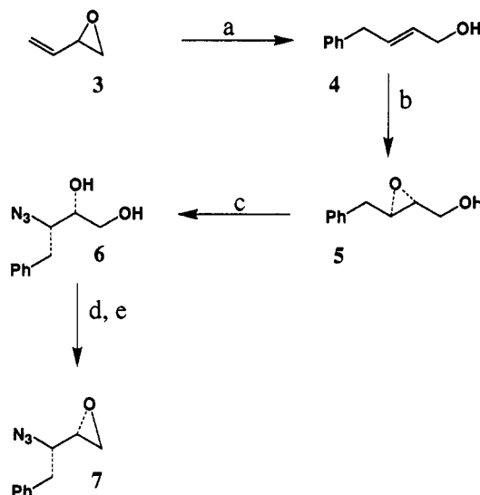
Scheme I. Synthesis of Azido Epoxide a
