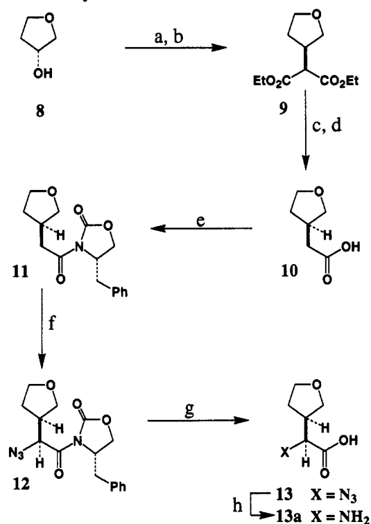
Scheme II. Synthesis of Amino Acid a
