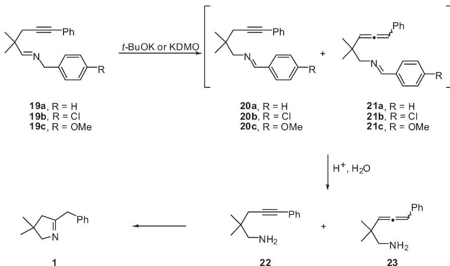
SCHEME 5 Synthesis of 1
