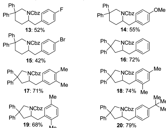
Scheme 3. Scope of Arene Incorporation a
