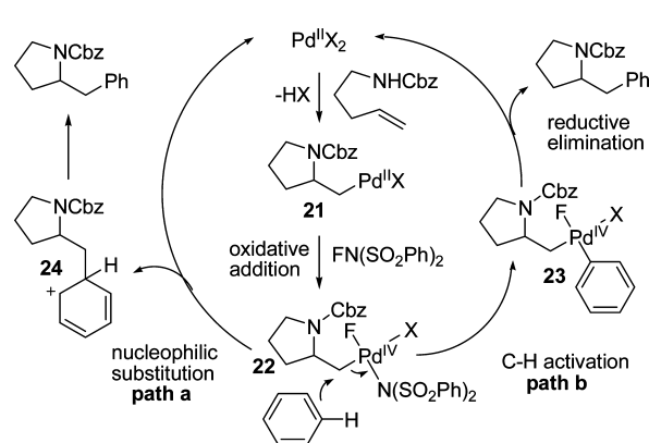
Scheme 4. Proposed Mechanistic Cycle
