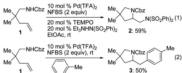
Scheme 1. Pd-Catalyzed Diamination Promoted by NFBS
