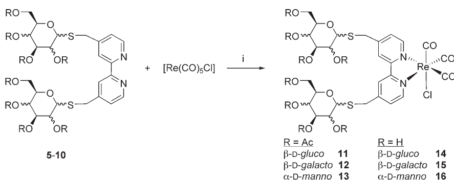
Scheme 2. Synthesis of the rhenium complexes: i) methanol, 10 h, reflux.
