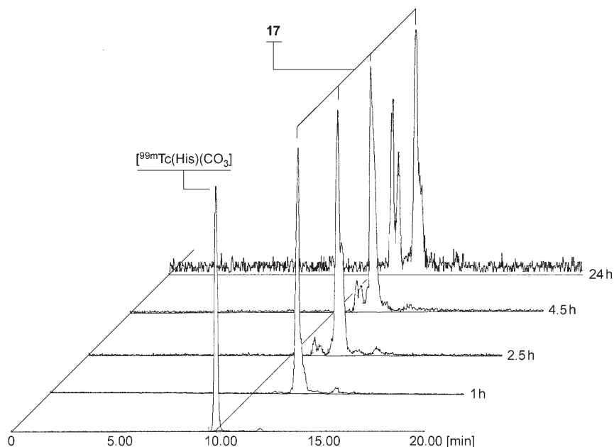
Figure 2. HPLC radiation traces for the histidine challenge experiment with 17 compared to the sample ^{99m}\text{Tc}-(\text{His})(\text{CO})_3 .
