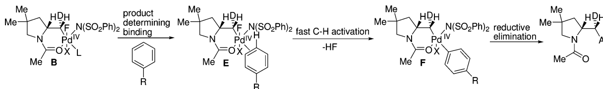
Figure 12. Mechanism for arene incorporation from Pd-alkyl complex.
