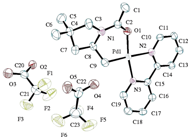
Figure 5. Crystal structure of bipy-Pd-alkyl [(\text{CF}_3\text{CO}_2)_2\text{H}] complex 10 . Bond distances (Å): Pd–O = 2.024, Pd–C = 2.010, Pd–N2 = 2.102, Pd–N3 = 2.206.
