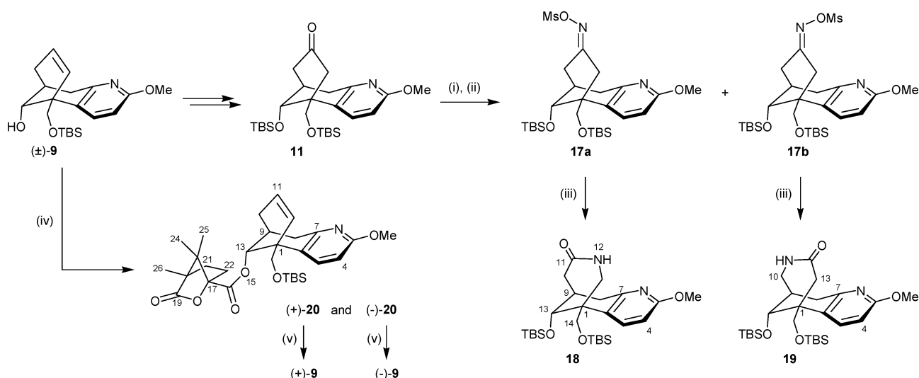
Scheme 3 Resolution of key intermediate 9 and initial analogue investigation. Reagents and conditions: (i) \text{NH}_2\text{OH}\cdot\text{HCl} , pyridine, \text{EtOH-H}_2\text{O} (1 : 1), reflux, 3 h, 91%; (ii) \text{MeSO}_2\text{Cl} , pyridine, DCM, -10^\circ\text{C} to r.t., 18 h, 94% 17a or 72% 17b ; (iii) aq. \text{KH}_2\text{PO}_4 (pH 7.4), THF, 76^\circ\text{C} , 20 h, 83% 18 or 84% 19 ; (iv) (1 S )-(–)-camphanic chloride, DMAP, DCM, 0^\circ\text{C} to r.t., 18 h, 34% (+)- 20 and 37% (–)- 20 ; (v) \text{K}_2\text{CO}_3 , MeOH, r.t., 24 h, 49% (+)- 9 or 41% (–)- 9 .
