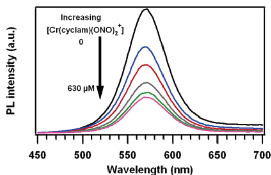
Figure 1. PL spectra ( \lambda_{\text{ex}} 366 nm) of water-soluble QDs ( \sim 130 nm) in phosphate buffer (15 mM, pH 8.2) with various concentrations of added 1 (0–630 \mu\text{M} ). PL intensities were corrected for the absorbance by 1 . The PL \lambda_{\text{max}} shifts slightly ( \sim 3 nm) to the red at the highest value of [ 1 ].
