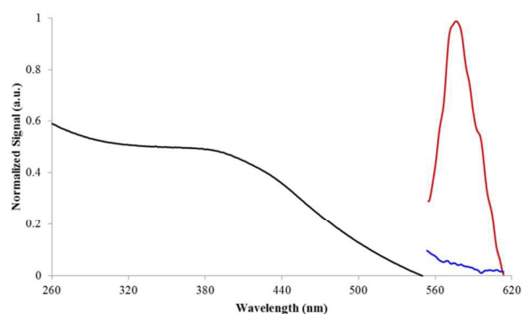
Fig. 5 Fluorescence emission spectra in water media ( \lambda_{\text{ex}} = 400 nm) of DHLA-capped HgSe NPs (line in red) and free DHLA (line in blue). The absorbance spectrum of the DHLA-capped HgSe NPs is also included (line in black).
