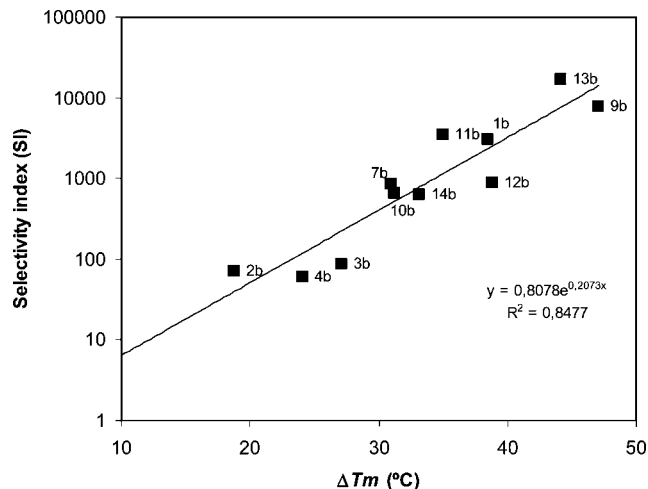
Figure 2. Plot of SI vs T_m for the bis(2-aminoimidazoline) compounds showing a good correlation between in vitro selectivity ( SI = (IC_{50} \text{ L6-cells})/(IC_{50} \text{ T. brucei}) ) and T_m increase: (■) 1b, 2b, 3b, 4b, 7b, 9b, 10b, 11b, 12b, 13b, and 14b.
