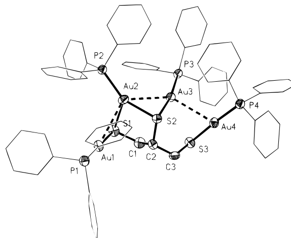
Figure 4. Structure of the cation in the crystal of \{[(\text{Ph}_3\text{P})\text{Au}]\text{S}(\text{CH}_2)\text{CHS}[\text{Au}(\text{PPh}_3)]_2\}^+\text{BF}_4^- 6 (ORTEP, except for phenyl carbon atoms; hydrogen atoms omitted for clarity). Selected distances [Å] and angles [deg]: Au1–Au2, 3.201(1); Au2–Au3, 3.227(1); Au3–Au4, 3.178(1); Au1–S1, 2.296(3); Au2–S1, 2.597(2); Au2–S2, 2.399(2); Au3–S2, 2.328(2); Au4–S3, 2.285(2); Au1–P1, 2.247(3); Au2–P2, 2.248(2); Au3–P3, 2.255(2); Au4–P4, 2.254(2); Au1–S1–Au2, 81.5(1); Au1–S1–C1, 103.0(3); Au2–S1–C1, 97.1(3); Au2–S2–C2, 103.8(3); P1–Au1–S1, 175.5(1); P2–Au2–S1, 123.7(1); P2–Au2–S2, 149.1(1); Au2–S2–Au3, 86.1(1); Au3–S2–C2, 102.7(3); P3–Au3–S2, 169.3(1); Au4–S3–C3, 101.7(3); P4–Au4–S3, 176.8(1).
