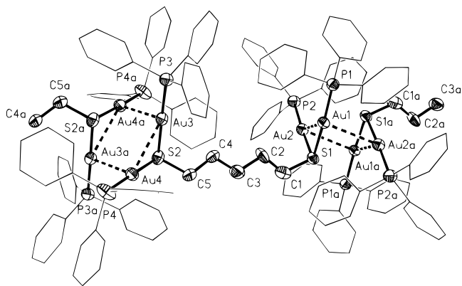
Figure 2. Part of a chain of \{[(\text{Ph}_3\text{P})\text{Au}]_2\text{S}(\text{CH}_2)_2\text{S}[\text{Au}(\text{PPh}_3)]_2\}^{2+} dications in the lattice of 3 (ORTEP, carbon atoms and hydrogen atoms omitted for clarity). Selected distances [Å] and angles [deg]: Au1–Au2a, 3.225(1); Au3–Au4a, 3.349(1); Au2–Au1–Au2a, 86.5(1); Au4–Au3–Au4a, 90.7(1).
