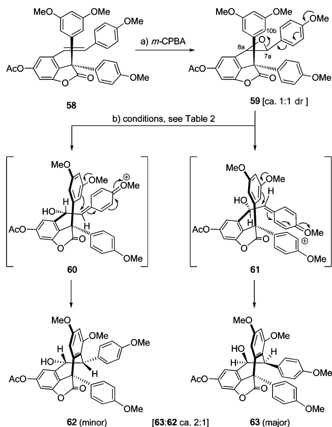
Scheme 7. Synthesis of Hexacyclic Hydroxy \gamma -Lactones 62 and 63 a
