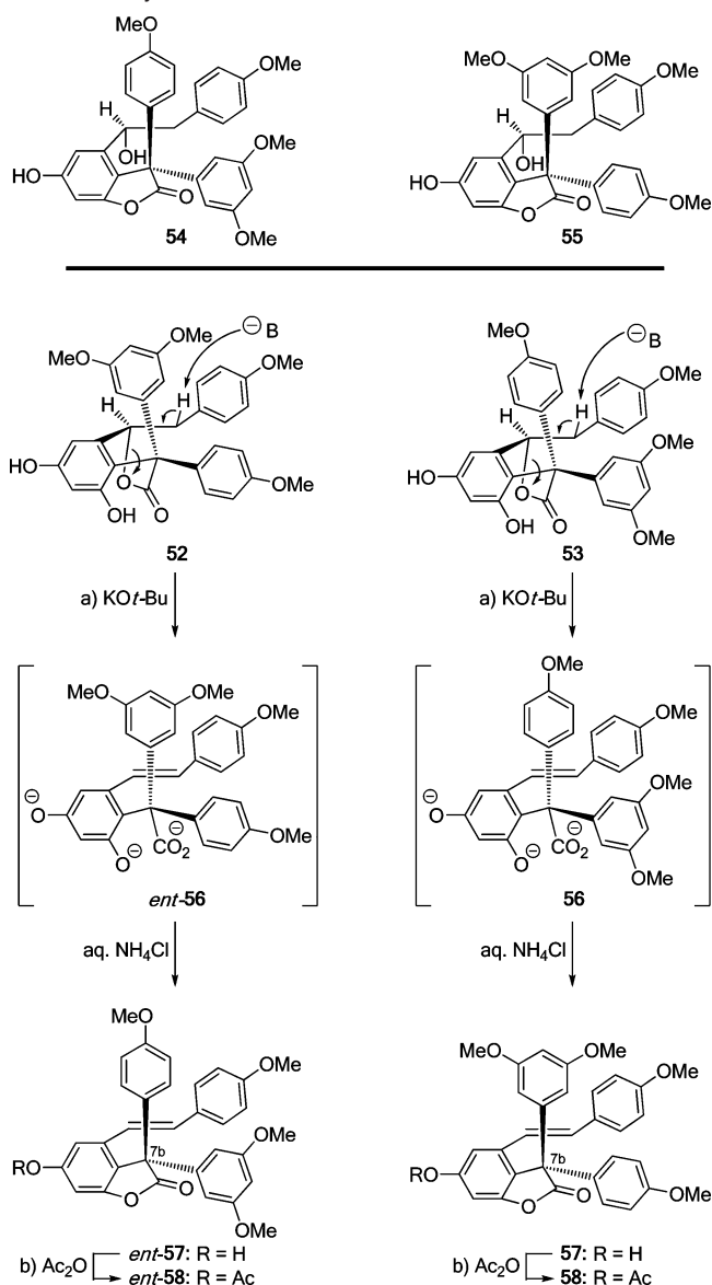
Scheme 6. Synthesis of Lactones ent - 58 and 58 a
