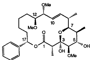
1 soraphen A
