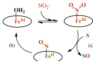
Scheme 1. Catalytic Cycle Where (a) the Water-Soluble \text{Fe}^{\text{III}}(\text{Por})(\text{NO}_2^-) Oxidizes Substrates To Form \text{Fe}^{\text{II}}(\text{Por})(\text{NO}) and (b) \text{Fe}^{\text{II}}(\text{Por})(\text{NO}) Spontaneously Regenerates \text{Fe}^{\text{III}}(\text{Por}) in the Absence of Oxygen a
