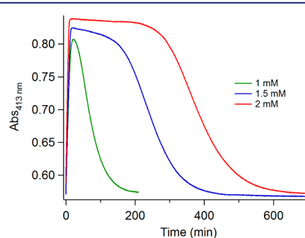
Figure 2. The temporal changes for the OAT reaction at pH 5.81 with \text{Fe}^{\text{II}}(\text{TPPS}) ( 1 , 8 \mu\text{M} ), \text{NaNO}_2 (10 mM), and several tppts concentrations (1–2 mM), showing fast initial formation of \text{Fe}^{\text{II}}(\text{TPPS})(\text{NO}) ( 2 , 413 nm) followed by slow reformation of 1 .
