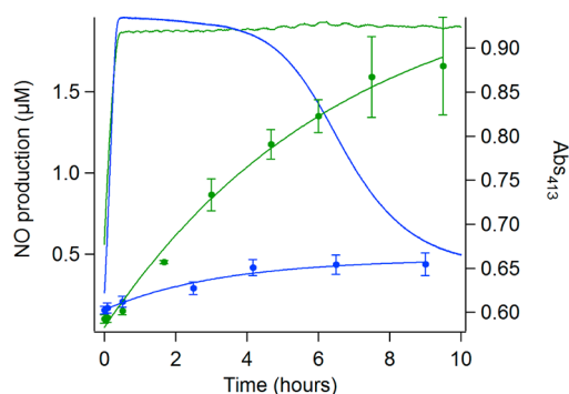
Figure 5. Reactions following addition of tppts (2.0 mM) or cysteine (1.0 mM), blue and green, respectively, to solutions of \text{Fe}^{\text{II}}(\text{TPPS}) (1, 10 \mu\text{M} ) and nitrite (10 mM) monitored by using the NOA to determine the NO formation (dots) and by the temporal absorbance at 413 nm, the \lambda_{\text{max}} of \text{Fe}^{\text{II}}(\text{TPPS})(\text{NO}) (2) (lines). The NO concentration in solution was calculated by determining that present in the gaseous head space and using the gas/aqueous solution partition coefficient to calculate [\text{NO}]_{\text{solution}} . (Note that a control reaction of tppts and nitrite without \text{Fe}(\text{TPPS}) did not lead to enhanced NO formation relative to nitrite solutions alone under the same conditions.)
