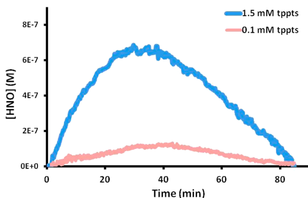
Figure 3. Temporal [\text{HNO}] detected using the cobalt-modified gold electrode 37 as generated by pH 5.81 buffered solutions containing \text{Fe}^{\text{III}}(\text{TPPS}) ( 1 , 8 \mu\text{M} ), \text{NaNO}_2 (10 mM), and \text{tppts} at 1.5 mM (blue) or 0.1 mM (pink). The supporting electrolyte was \text{NaNO}_3 (0.1 M). The plots are the average of two independent runs (see Figure S-9 for the individual raw data).
