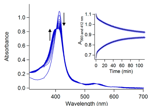
Figure 6. The reaction of \text{Fe}^{\text{II}}(\text{TPPS}) (5, 10 \mu\text{M} ) and nitrite (6.6 mM) at pH 5.81 (50 mM phosphate) as monitored by the absorbance changes. The reaction proceeds from 5 (412 nm) to form a broad band due to the formation of a 1:1 ratio of \text{Fe}^{\text{II}}(\text{TPPS})(\text{NO}) (2, 413 nm) and \text{Fe}^{\text{III}}(\text{TPPS}) (1, 393 nm). Inset: Temporal absorption changes at 413 nm (above) and 393 nm.
