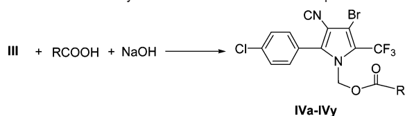
Scheme 2. General Synthetic Route of the Title Compounds IVa–IVy
