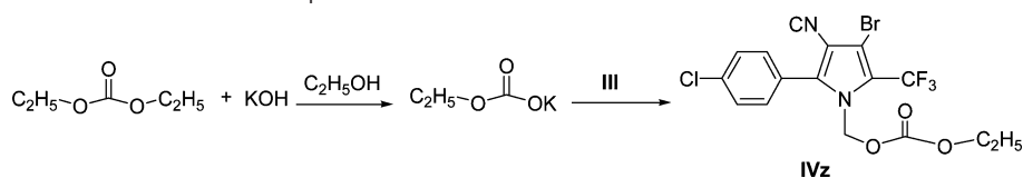
Scheme 3. General Synthetic Route of the Title Compound IVz
