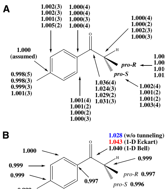
Figure 2. (A) Experimental ^{13}\text{C} KIEs ( k_{12\text{C}}/k_{13\text{C}} ) for the (–)-DIP-Cl reduction of 4'-methylphenyl isopropyl ketone. (B) Computed KIEs based on the [B3LYP/6-31G(d)] transition structure for Re attack.
