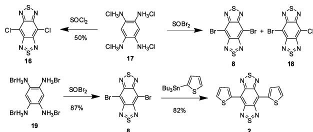
Scheme 3. Synthesis of 4,8-Disubstituted BBT via TAB
