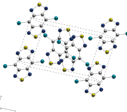
Figure 3. Crystal structure of 16 . Monoclinic, P2_1/n , a = 3.8426 Å, b = 7.4348 Å, c = 15.2226 Å, \beta = 90.339^\circ , V = 434.88(6) Å 3 , Z = 2 , \rho_{\text{calcd}} = 2.01 g/cm 3 .
