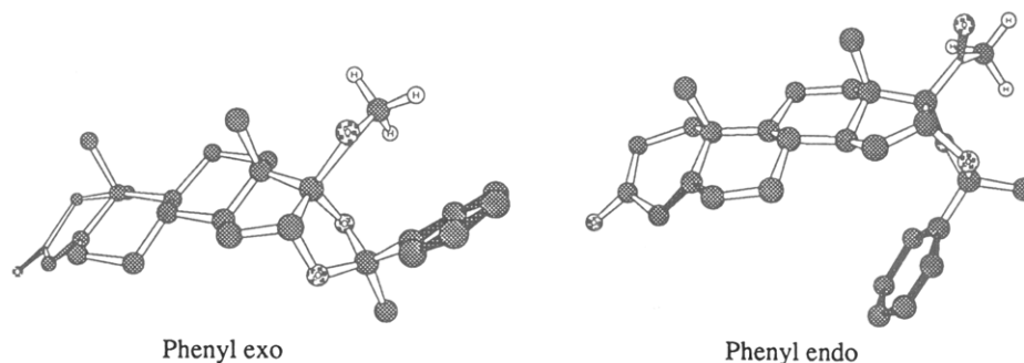
Figure 3. Two diastereomers of 16 \alpha ,17 \alpha -[1'-phenyl(ethylenedioxy)]pregn-4-ene-3,20-dione. The phenyl exo diastereomer exhibits shielding of the 21-CH 3 resonance in 1 H NMR. The structure of the phenyl endo diastereomer was obtained by retrieval of the crystal structure of 21-bromo-9 \alpha -fluoro-11 \beta -hydroxy-16 \alpha ,17 \alpha -[ \beta -methyl- \alpha -phenyl(methylenedioxy)]-4-pregnene-3,20-dione from the Cambridge Structural Database, conversion of the proper heteroatoms to protons and energy minimization in Macromodel version 3.1 13 (MM2 14 force field). The phenyl exo isomer was obtained by isomerization at the 2' center, followed by minimization (MM2 14 force field).
