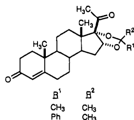
Figure 2. 16α,17α-(Methylenedioxy)progesterone derivatives that demonstrate in vivo progestational activity. 8 labeling of the PgR. The Roussel-Uclaf compound, promegestone (R5020, Figure 1), is currently the most widely used PAL reagent for the PgR, in spite of displaying photocovalent attachment efficiencies of only 2–5%. 4a While low photoattachment efficiencies may be sufficient for identifying some sites of ligand-receptor contact, more efficient photocovalent attachment may be necessary to identify other residues in the PgR hormone binding domain that are critical for ligand binding.
