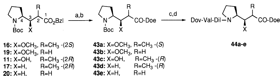
Chart 6. Synthesis of Analogs Modified at the Dil Unit
