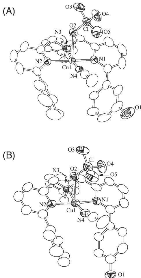
Figure 3. ORTEP drawings of (A) \text{Cu}^{\text{II}}\text{L}^{\text{m}}\text{H} and (B) \text{Cu}^{\text{II}}\text{L}^{\text{p}}\text{H} showing 50% probability thermal ellipsoids. Hydrogen atoms are omitted for clarity.
