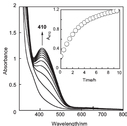
Figure 5. Spectral change of the aerobic reaction of \text{Cu}^{\text{II}}\text{L}''\text{H} (0.5 mM) in methanol containing \text{Et}_3\text{N} (1.0 mM) at 60 °C in a UV cell with a path length of 1.0 cm. Inset: The time course of the absorption change at 410 nm.
