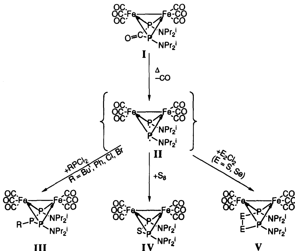
Fig. 1. General scheme for the reactions of (^i\text{Pr}_2\text{NP})_2\text{COFe}_2(\text{CO})_6 with \text{R-PCl}_2 ( \text{R} = ^i\text{Bu}, \text{Ph}, \text{Cl}, \text{Br} ), \text{S}_8 , and \text{E}_2\text{Cl}_2 ( \text{E} = \text{S}, \text{Se} ).
