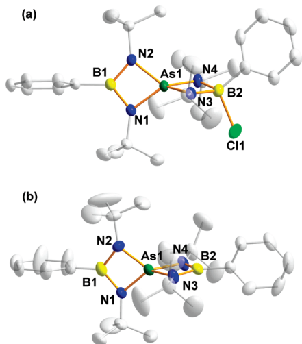
Figure 3. (a) Molecular structure of [PhB( \mu -N'Bu) _2 As( \mu -N'Bu) _2 B(Cl)Ph] ( 3 ) and (b) crystal structure of the [PhB( \mu -N'Bu) _2 ] _2 As ^+ cation in 4 with the atomic numbering schemes. Hydrogen atoms have been omitted for clarity. Only one of the two independent cations is shown in 4 .
