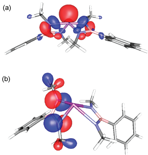
Figure 1. SOMOs (isosurface value \pm 0.06 ) of the neutral [PhB(μ-NMe) 2 ] 2 M • radicals; (a) M = P, As, Sb; (b) M = Bi. Electronic structures of the t Bu-derivatives, [PhB(μ-N'Bu) 2 ] 2 M • (M = P, As, Sb, Bi), are analogous to that presented in Figure 1a.
