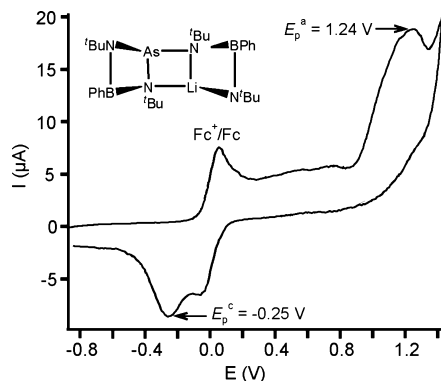
Figure 5. Cyclic voltammogram of 1b (1.4 mM) and ferrocene (0.6 mM) in THF at a Au electrode at 21 °C, [nBu _4 N][PF _6 ] (0.4 M), \nu = 0.2 V s ^{-1} .
