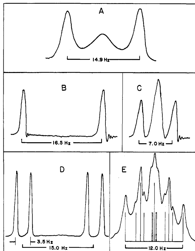
Figure 1.—Hydrogen-1 spectra: (a) \text{P}(\text{NCH}_3\text{NCH}_3)_3\text{P} ; (b) \text{ClP}(\text{NCH}_3\text{NCH}_3)_2\text{PCl} ; (c) \text{Cl}_2\text{PNCH}_3\text{NCH}_3\text{PCl}_2 ; (d) \text{FP}(\text{NCH}_3\text{NCH}_3)_2\text{PF} ; (e) \text{F}_2\text{PNCH}_3\text{NCH}_3\text{PF}_2 ; compared to a line spectrum calculated using the parameters described in the text.
