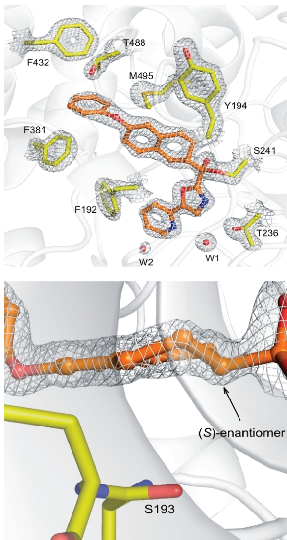
Figure 8. (top) View of 12 in the binding pocket of FAAH and its interactions. (bottom) An enlarged view of the chiral center within the tetrahydronaphthalene is shown. Electron density at 1.5 \sigma contour is shown with white meshes.
