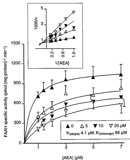
Figure 3 Mode of inhibition of [\text{H}]\text{-AEA} metabolism in rat brain membranes by palmitoylethylamide (PA-Et). Means \pm s.e.mean of three experiments are shown in the main plot. A secondary Lineweaver-Burk replot of the mean data is shown in the insert to illustrate the mixed-type nature of the inhibition. The K_{i(\text{slope})} and K_{i(\text{intercept})} values were calculated from the mean data as described in Methods.
