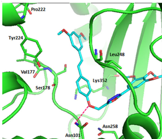
Fig. 2. Molecular docking poses of compound 9b at the colchicine binding site of tubulin
