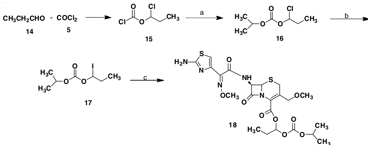
Scheme-V: Synthetic route of propyl analogue of cefpodoxime proxetil (18); Reagents: (a) isopropanol, pyridine (b) sodium iodide, toluene (c) cefpodoxime acid, DBU, DMAc, toluene, cyclohexane, water; Origin: Presence of propanaldehyde in acetaldehyde used during the preparation of 1-chloroethyl chloroformate (6) may give propyl analogue of cefpodoxime proxetil (18) in the subsequent steps of cefpodoxime proxetil; Control: Propanaldehyde should be controlled to not detected level in acetaldehyde used during the preparation of 1-chloroethyl chloroformate (6)
