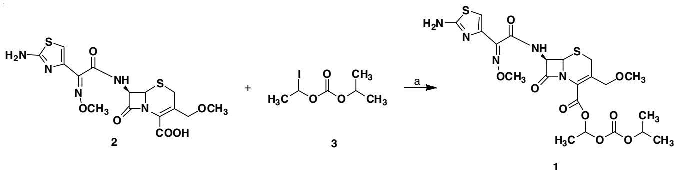
Scheme-I: Synthetic route of cefpodoxime proxetil ( 1 ); Reagents: (a) DBU, DMAC, toluene and cyclohexane
