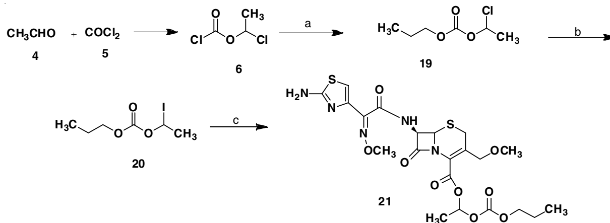
Scheme-VI: Synthetic route of N -propyl analogue of cefpodoxime proxetil ( 21 ); Reagents: (a) N -propanol, pyridine (b) sodium iodide, toluene (c) cefpodoxime acid, DBU, DMAc, toluene, cyclohexane, water; Origin: Presence of N -propanol in isopropanol used during the preparation of 1-chloro ethyl isopropyl carbonate ( 7 ) may give N -propyl analogue of cefpodoxime proxetil ( 21 ) in the subsequent steps of cefpodoxime proxetil; Control: N -propanol should be controlled to not detected level in isopropanol used during the preparation of 1-chloroethyl isopropyl carbonate ( 7 )
