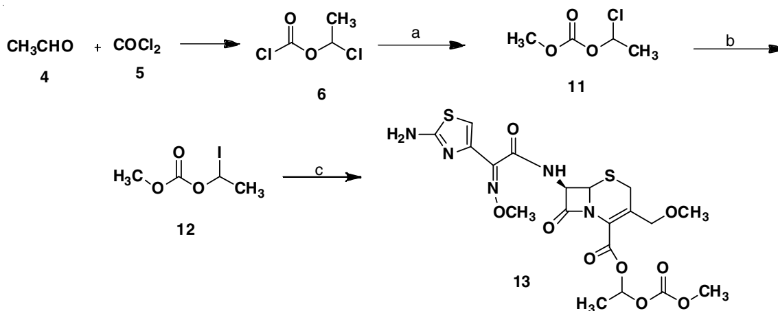
Scheme-IV: Synthetic route of methyl analogue of cefpodoxime proxetil (13); Reagents: (a) ethanol, pyridine (b) sodium iodide, toluene (c) cefpodoxime acid, DBU, DMAc, toluene, cyclohexane, water; Origin: Presence of methanol in isopropanol used during the preparation of 1-chloroethyl isopropyl carbonate (7) may give methyl analogue of cefpodoxime proxetil (13) in the subsequent steps of cefpodoxime proxetil; Control: Methanol should be controlled to not detected level in isopropanol used during the preparation of 1-chloroethyl isopropyl carbonate (13)
