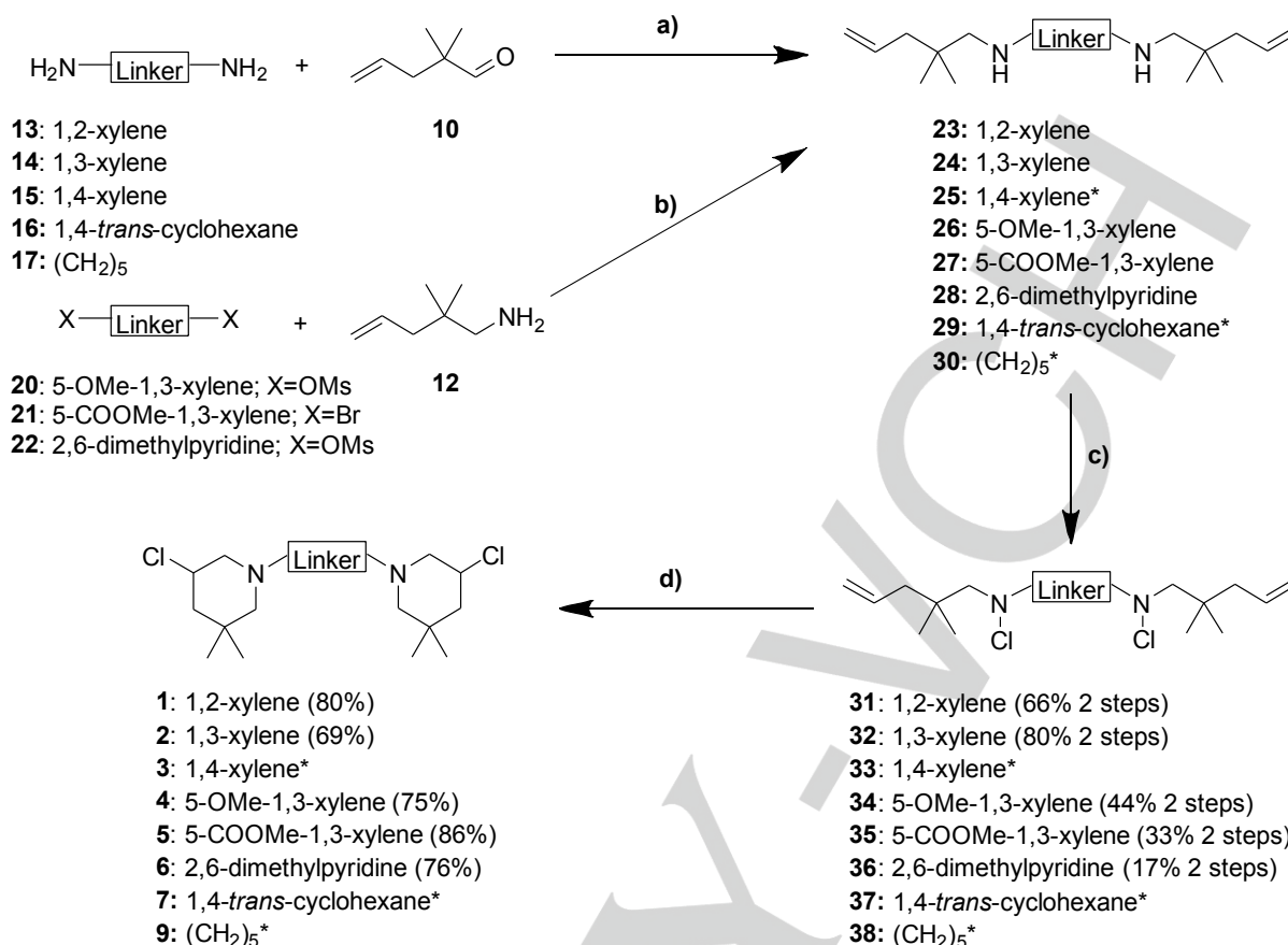
Scheme 1. Synthesis of bis -3-chloropiperidines 1-6 . Reactants and conditions: a) NaBH(OAc) 3 , AcOH, dry DCM, 0°C to rt, 16-18 h; b) NaH, dry THF, 0°C to rt, 20-22 h; c) NCS, dry DCM, 0°C to rt, 2.5-3 h; d) TBAI (cat.), dry CHCl 3 , 60°C (oil bath temperature), 2-2.5 h (inseparable diastereomeric mixture). *The synthesis of compounds 3 , 7 and 9 as well as their corresponding precursors has been described elsewhere. [4b]
