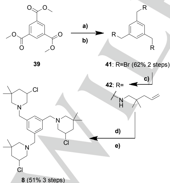
Scheme 2. Synthesis of tris -3-chloropiperidine 8 . Reactants and conditions: a) LAH, dry THF, 0°C to rt to reflux, 18 h; b) PBr 3 , dry Et 2 O, 0°C to rt, 24 h; c) 2,2-dimethylpent-4-en-1-amine 12 , dry DCM, 0°C to rt, 68 h; d) NCS, dry DCM, 0°C to rt, 2.5 h; e) TBAI (cat.), dry CHCl 3 , reflux, 4 h.
