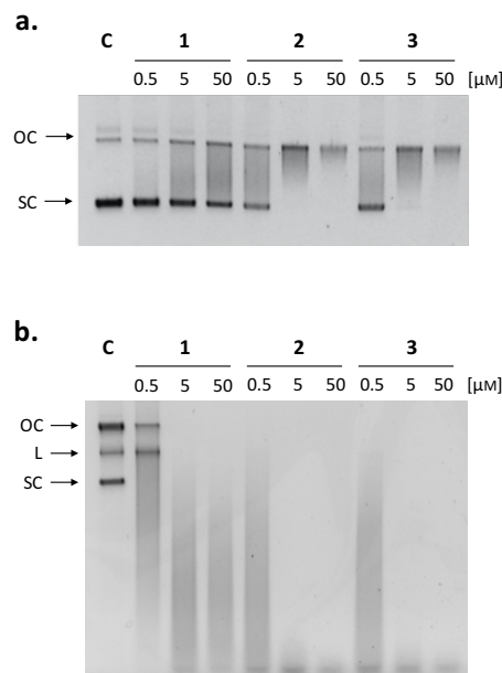
Figure 3. DNA cleavage assay for compounds 1 , 2 and 3 . DNA cleavage assay upon incubation with pBR322 after 3 h (a) and 18 h (b) at 37 °C at increasing compound concentrations (0.5, 5, 50 μM). SC: supercoiled plasmid; L: linearized plasmid; OC: open circular plasmid; C: supercoiled pBR322 plasmid control.
