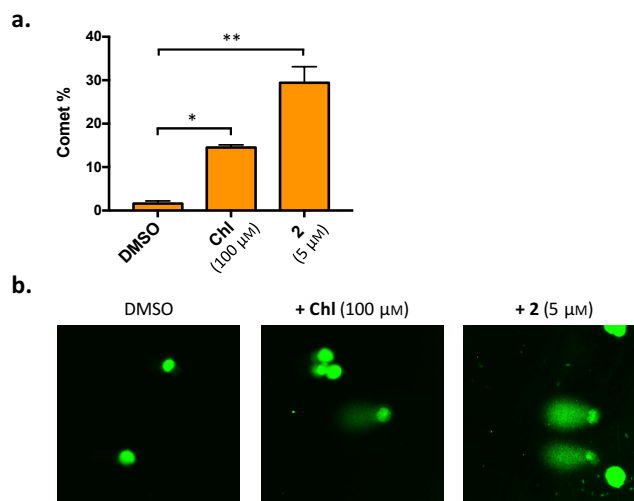
Figure 6. Alkaline Single-Cell Gel Electrophoresis (SCGE) assay. Alkaline SCGE assay was performed on BxPC-3 cells upon incubation with DMSO 0.5%, chlorambucil (Chl) and compound 2 for 6 h at the indicated concentrations. (a) The bar chart reports the relative percentage of comets (n° cells forming a comet /total n° of cells) detected in two randomly captured fields from two independent experiments per condition. (b) Representative images (40x) of treated samples (including negative and positive controls) with comets are also reported. Paired t-test: * p < 0.05 ** p < 0.001
