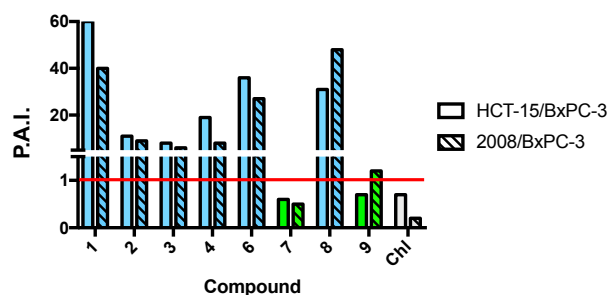
Figure 4. Preferential activity indexes (P.A.I.) of 3-chloropiperidines. P.A.I. are expressed as ratio between the compound MTT IC 50 against HCT-15 and BxPC-3 cells (solid bars), as well as 2008 and BxPC-3 cells (dashed bars). Chl: Chlorambucil. Green bars: aliphatic B-CePs; blue bars: aromatic B-CePs; grey bar: Chl.
