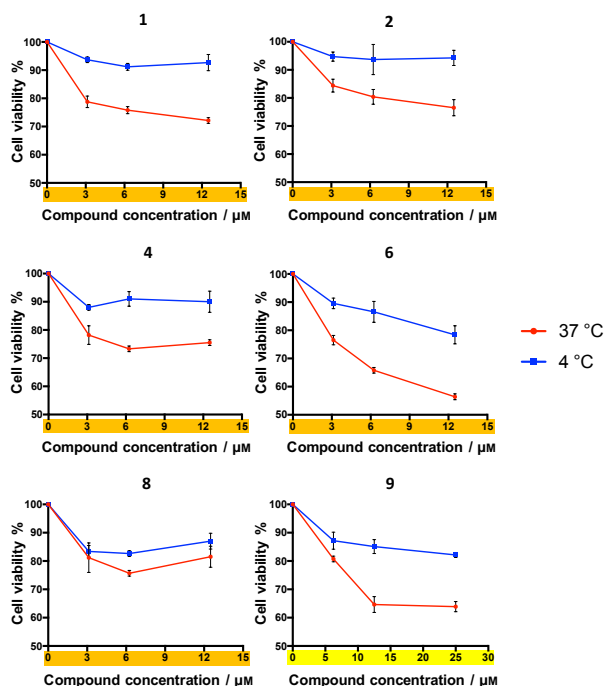
Figure 5. Cell viability curve for BxPC-3 cells upon treatment at 37 °C vs 4 °C with test compounds ( 1 , 2 , 4 , 6 , 8 , 9 ). BxPC-3 cell viability upon exposure to increasing concentrations of selected compounds (from 3 μM to 12 μM of rigid derivatives 1 , 2 , 4 , 6 , 8 and from 10 μM to 50 μM of 9 ) for 5 h at 37 °C (red curve) or 4 °C (blue curve), followed by a gentle rinse of wells with PBS and addition of fresh RPMI medium. The MTT assay was performed at 72 h.
