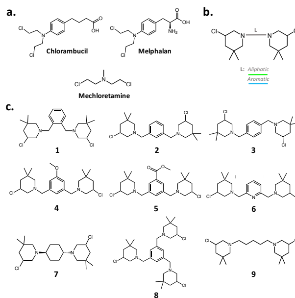
Figure 1. (a) Chemical structure of chlorambucil, melphalan and mechlorethamine. (b) General structure of B-CePs. Different connecting linkers (L) are schematized with different colors. Green line: aliphatic linkers; blue line: aromatic linkers. (c) Chemical structures of the analyzed 3-chloropiperidines.
