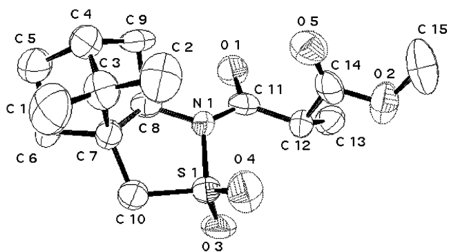
FIGURE 2. ORTEP drawing of compound 2j (major diastereoisomer).
