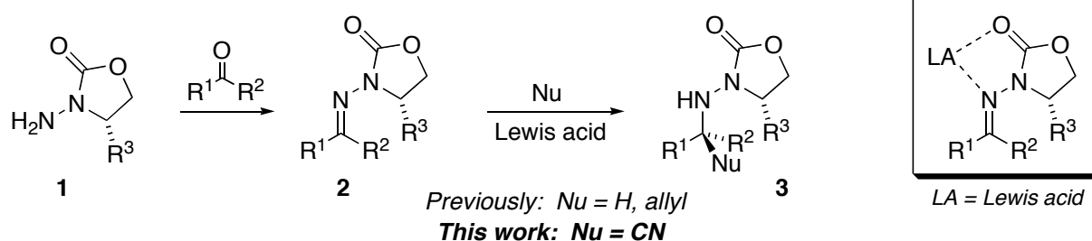
Scheme 2. General chiral N -acylhydrazone approach
