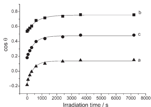
Figure 3. Contact angle variation during photolysis using soft UV light (365 nm, 7 \text{ mW cm}^{-2} ). a) Advancing water contact angle, b) receding water contact angle, and c) the average of the advancing and receding water contact angle. In cases (a) and (b) the lines are guides to the eye whilst in case (c) the line represents a fit to the data using the Cassie equation (see text).
