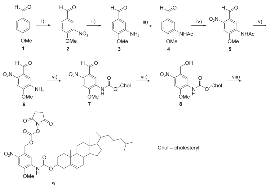
Scheme 1. Synthesis of the photocleavable tether 9 . i) 70% \text{HNO}_3 , 90%; ii) Raney \text{Ni}/\text{NH}_4\text{Cl}/\text{H}_2\text{O} , 80%; iii) acetic anhydride/acetic acid, 95%; iv) 70% \text{HNO}_3 , 75%; v) 2 N \text{HCl} , 70%; vi) cholesteryl chloroformate/diisopropylethylamine/DMAP/toluene, 55%; vii) \text{NaBH}_4/\text{THF} , 90%; viii) N,N' -disuccinimidyl carbonate/triethylamine/DMF, 85%. ^1\text{H} and ^{13}\text{C} NMR Spectra of compounds 3–9 are available in the Supporting Information.
