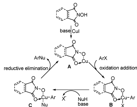
SCHEME 1. Proposed Mechanism for the Coupling Reaction
