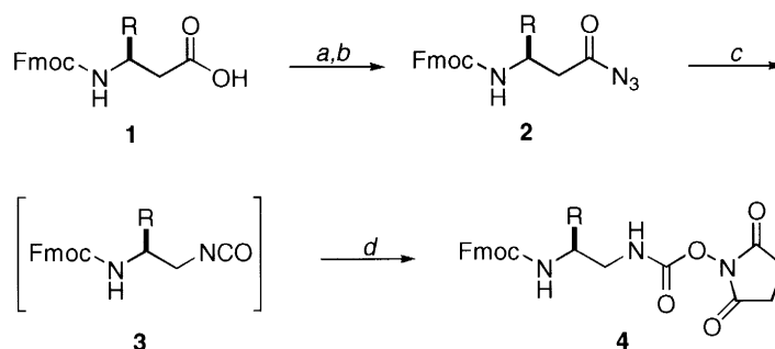
Scheme 1. (a) EtOCOCl, NMM, THF, -15°C, 15 min; (b) NaN 3 , H 2 O, 5 min; (c) toluene, 65°C; (d) N -hydroxysuccinimide, pyridine, 65°C, 5 min
