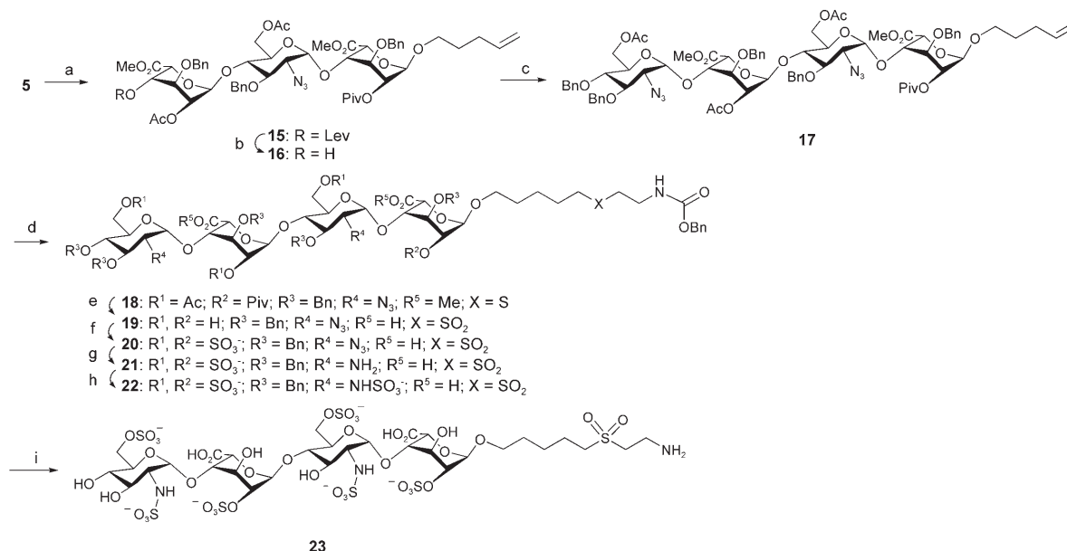
Scheme 4. Assembly of tetrasaccharide 23 . a) 2 , TMSOTf (cat.), \text{CH}_2\text{Cl}_2 , -20^{\circ}\text{C} , 4 Å MS, 91%; b) \text{H}_2\text{NNH}_2\cdot\text{H}_2\text{O} , Py/AcOH, \text{CH}_2\text{Cl}_2 , 86%; c) 3 , TMSOTf (cat.), \text{CH}_2\text{Cl}_2 , -20^{\circ}\text{C} , 4 Å MS, 88%; d) \text{HS-CH}_2\text{-CH}_2\text{-NH}_2 , AIBN, THF, 75^{\circ}\text{C} , 61%; e) LiOH, \text{H}_2\text{O}_2 ; KOH, MeOH, 88%; f) \text{SO}_3\cdot\text{Et}_3\text{N} , DMF, 55^{\circ}\text{C} , 80%; g) \text{PMe}_3 , THF, NaOH, quant.; h) \text{SO}_3\cdot\text{Py} , Py, TEA, 78%; i) \text{H}_2 , Pd/C, quant.
