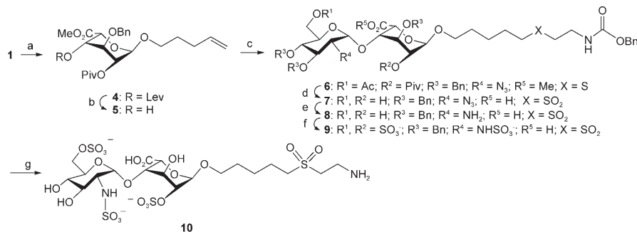
Scheme 2. Synthesis of disaccharide 10 . a) 4-Penten-1-ol, TMSOTf, CH 2 Cl 2 , -25°C, 81%; b) H 2 NNH 2 ·H 2 O, Py/AcOH, CH 2 Cl 2 , 91%; c) 3 , TMSOTf, CH 2 Cl 2 , -25°C, 81%; HS(CH 2 ) 3 NH 2 , AIBN, THF, 75°C, 78%; d) LiOH, H 2 O 2 ; KOH, MeOH, 73%; e) PMe 3 , THF, NaOH, 89%; f) SO 3 ·Py, Py, 87%; g) H 2 , Pd/C, quant.
