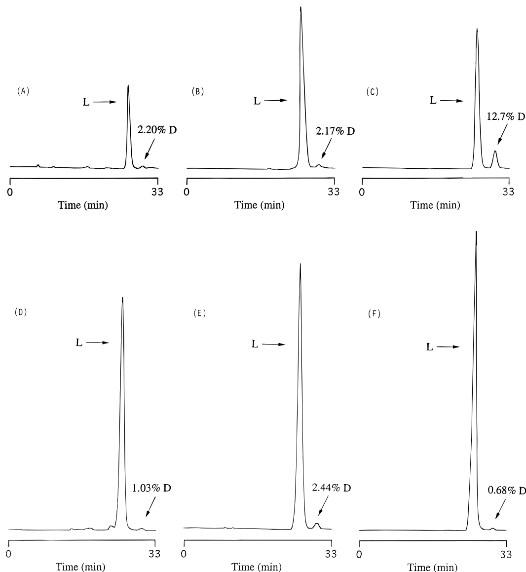
Figure 5. Determination of enantiomeric composition of theanine in tea samples using FMO-C-Gly-Cl derivatizing agent and the column switching technique. Column: \gamma -CD (used in the polar-organic mode; see Table 3 for chromatographic conditions). Flow rate: 1 mL/min. Detection: fluorescence, \lambda_{\text{ex}} = 266 nm and \lambda_{\text{em}} = 315 nm. Samples (see Table 4): (A) Sencha (green) tea, (B) Gunpowder (green) tea, (C) Formosa Oolong (half-green) tea, (D) Lapsang Souchong (black) tea, (E) Rosen (black) tea, and (F) Keemun FOP (black) tea.
